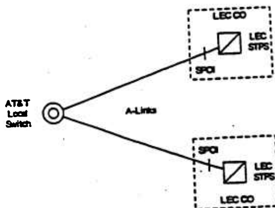
Figure 6. A-Link Interface
