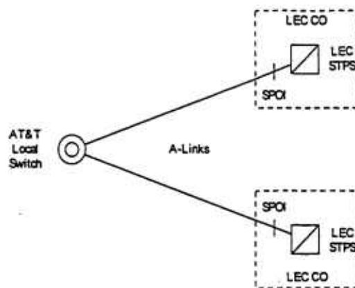
Figure 6. A-Link Interface
