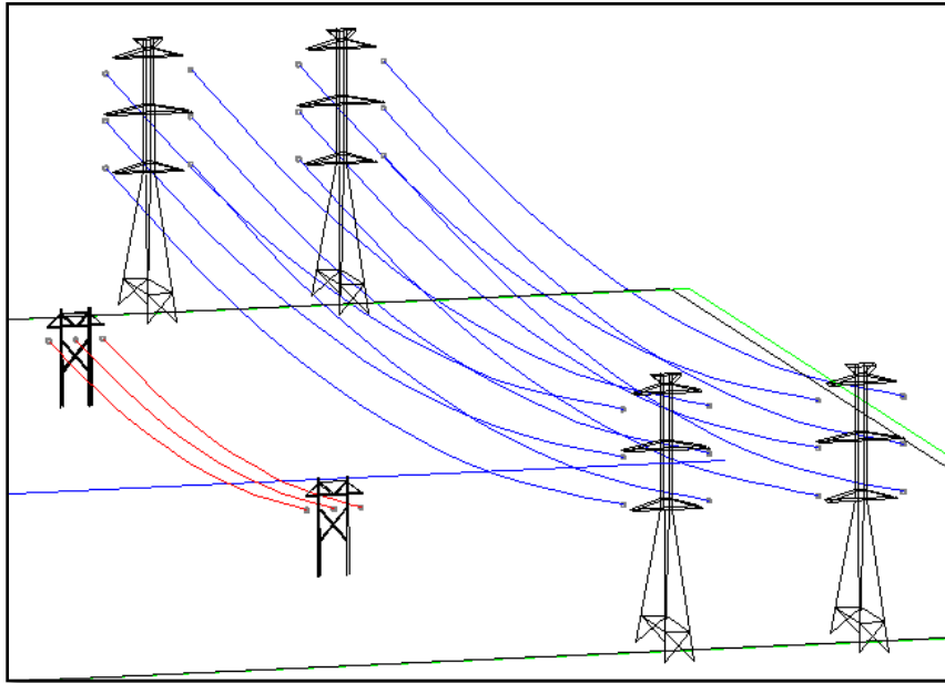
Figure 13. Existing A Line (left) and Con Ed Transmission lines (right)
