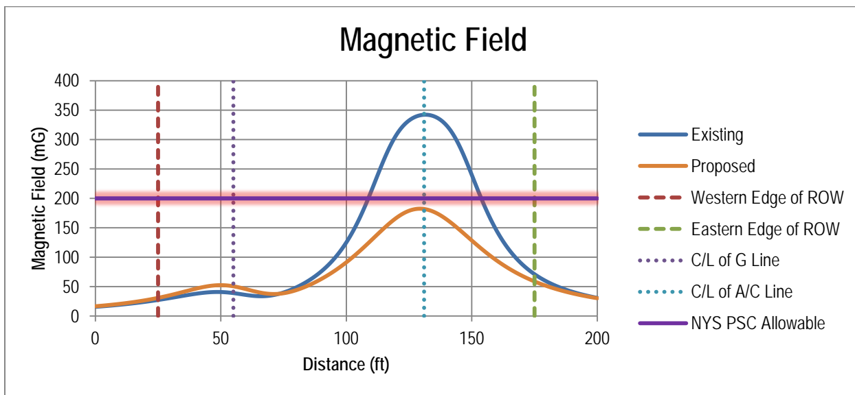
Figure 11. MF Levels on ROW with G and A and C Lines
