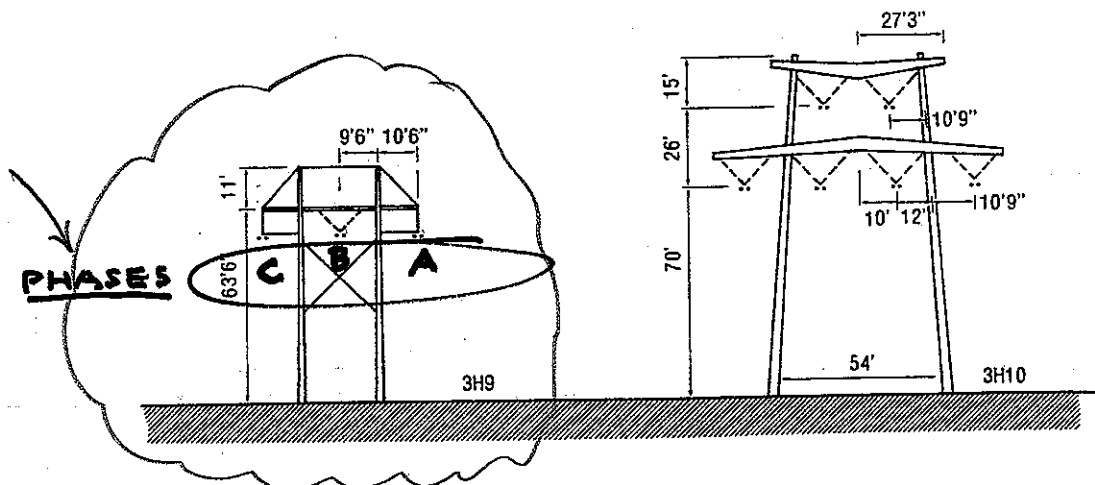
Figure 2.7.3. Typical H-frame-type structures for 345-kV transmission systems.
