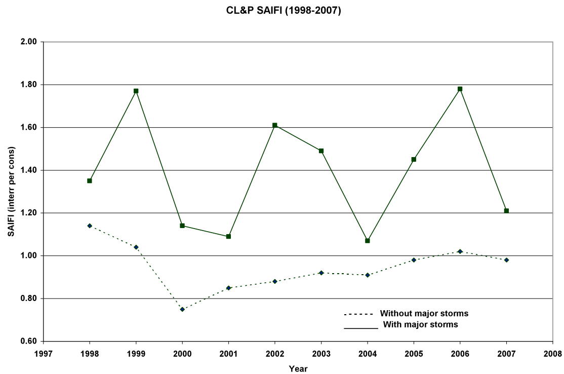
Figure 5: CL&P SAIFI (1998-2007)
