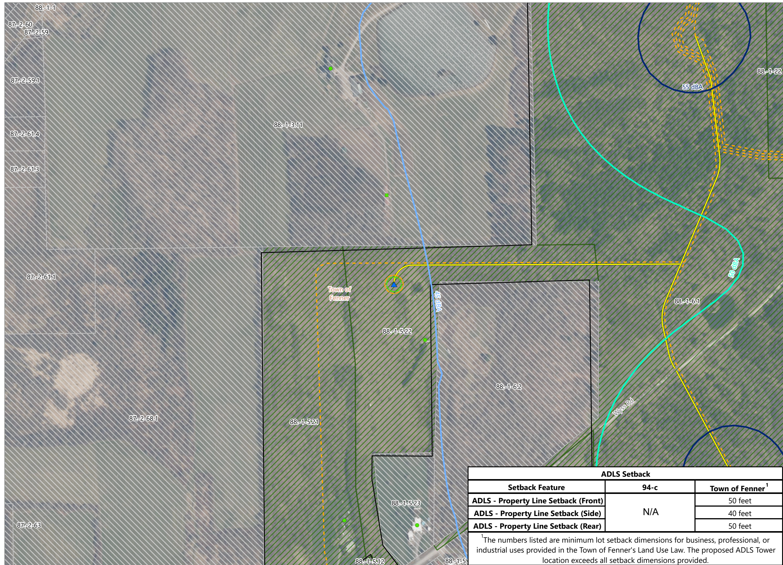
Figure 24-1. Wind Turbine Setbacks - Revision 2 ADLS Tower
