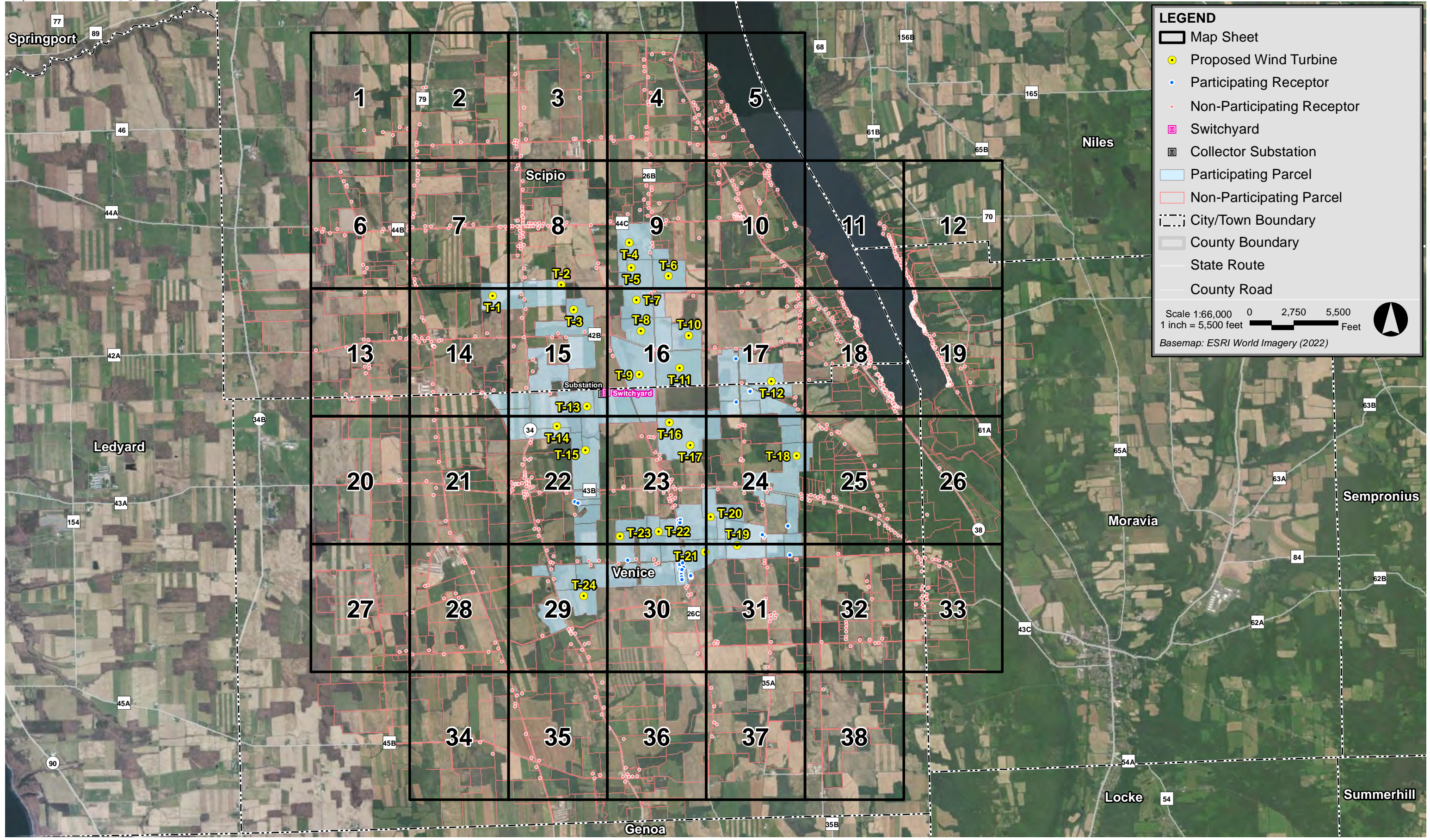
Figure 5-1, Index Shadow Flicker Modeling Locations
