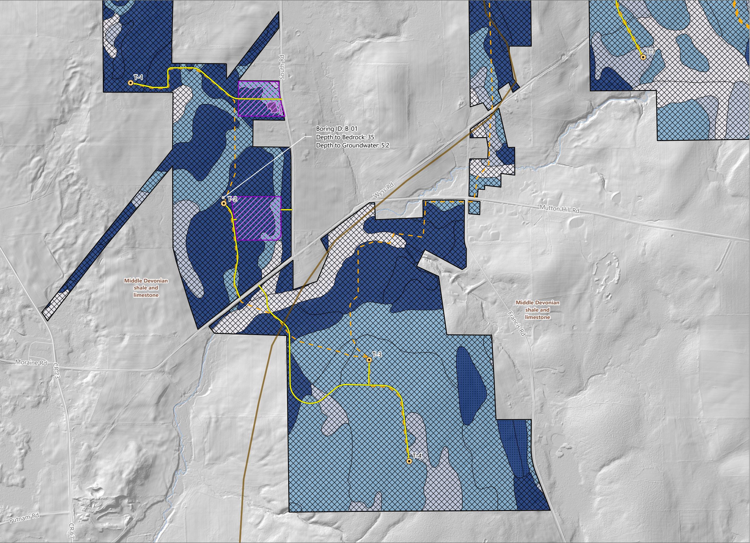
Figure 10-4. Bedrock
