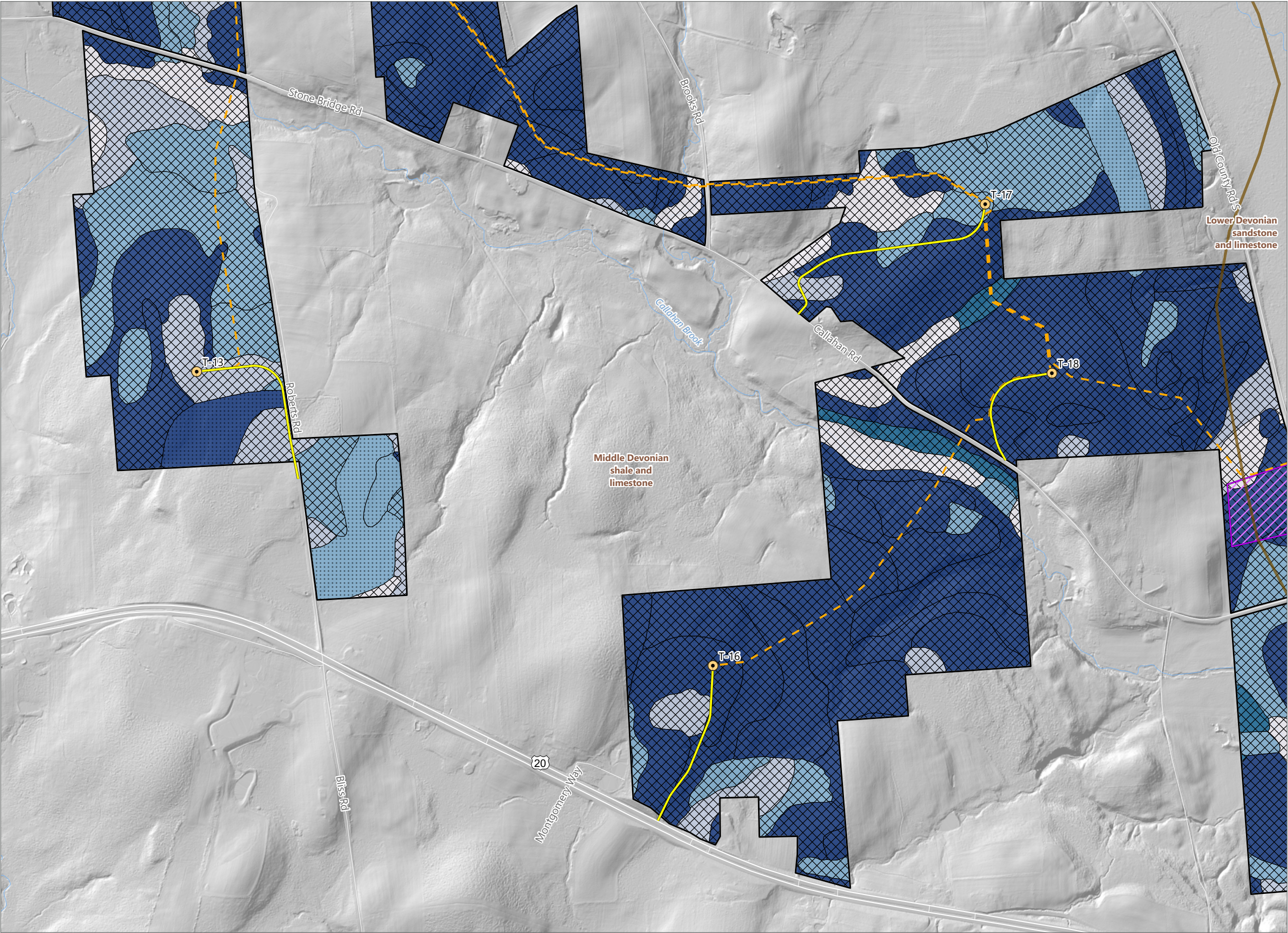
Figure 10-4. Bedrock
