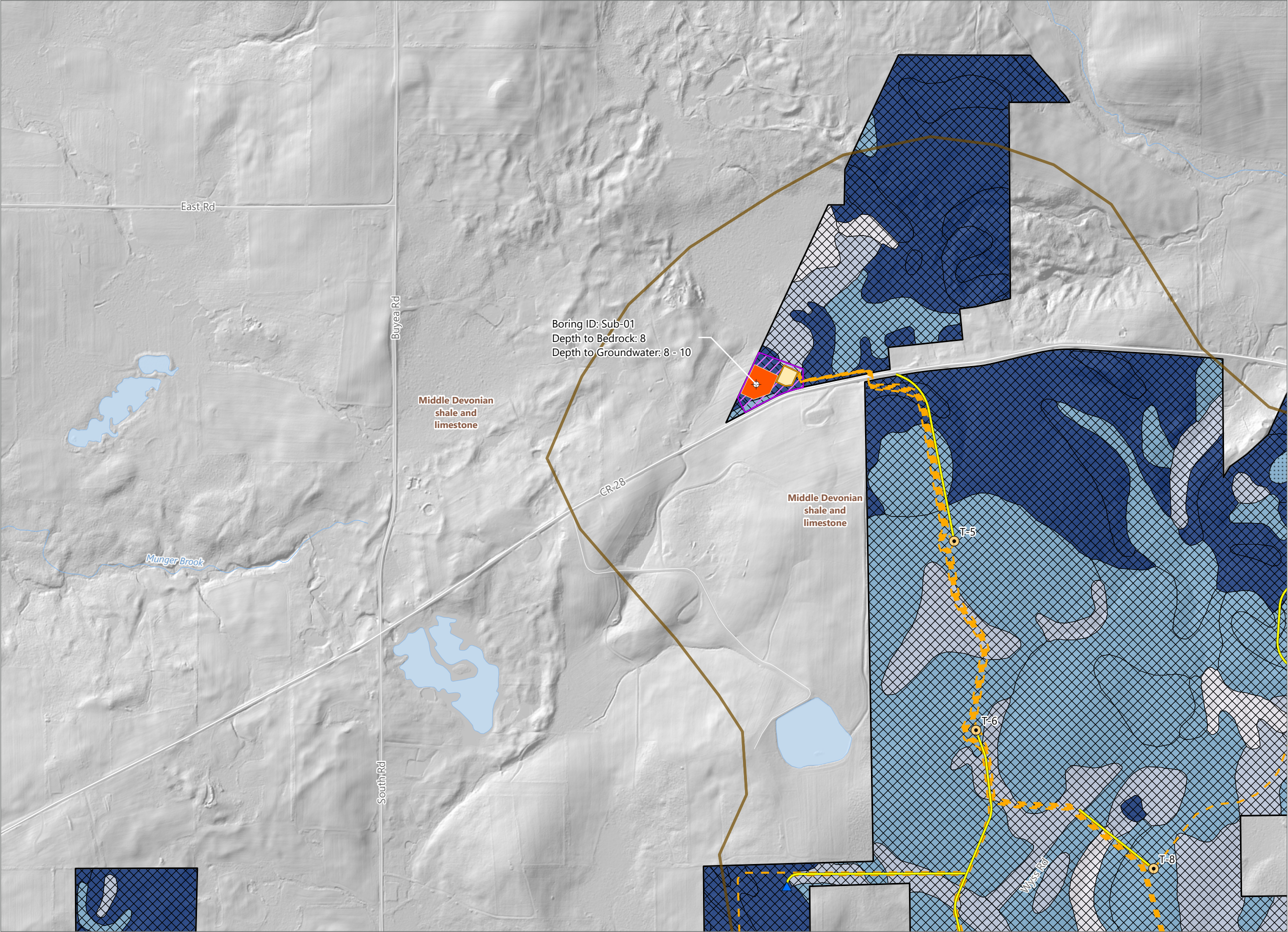
Figure 10-4. Bedrock
