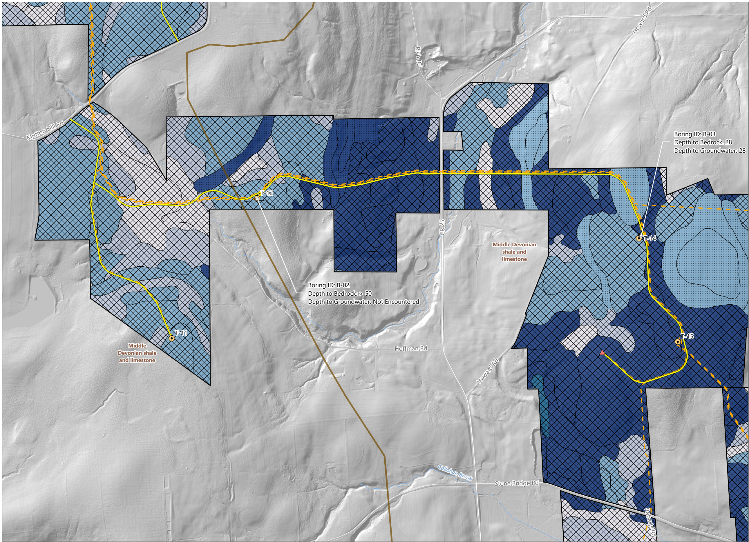
Figure 10-4. Bedrock
