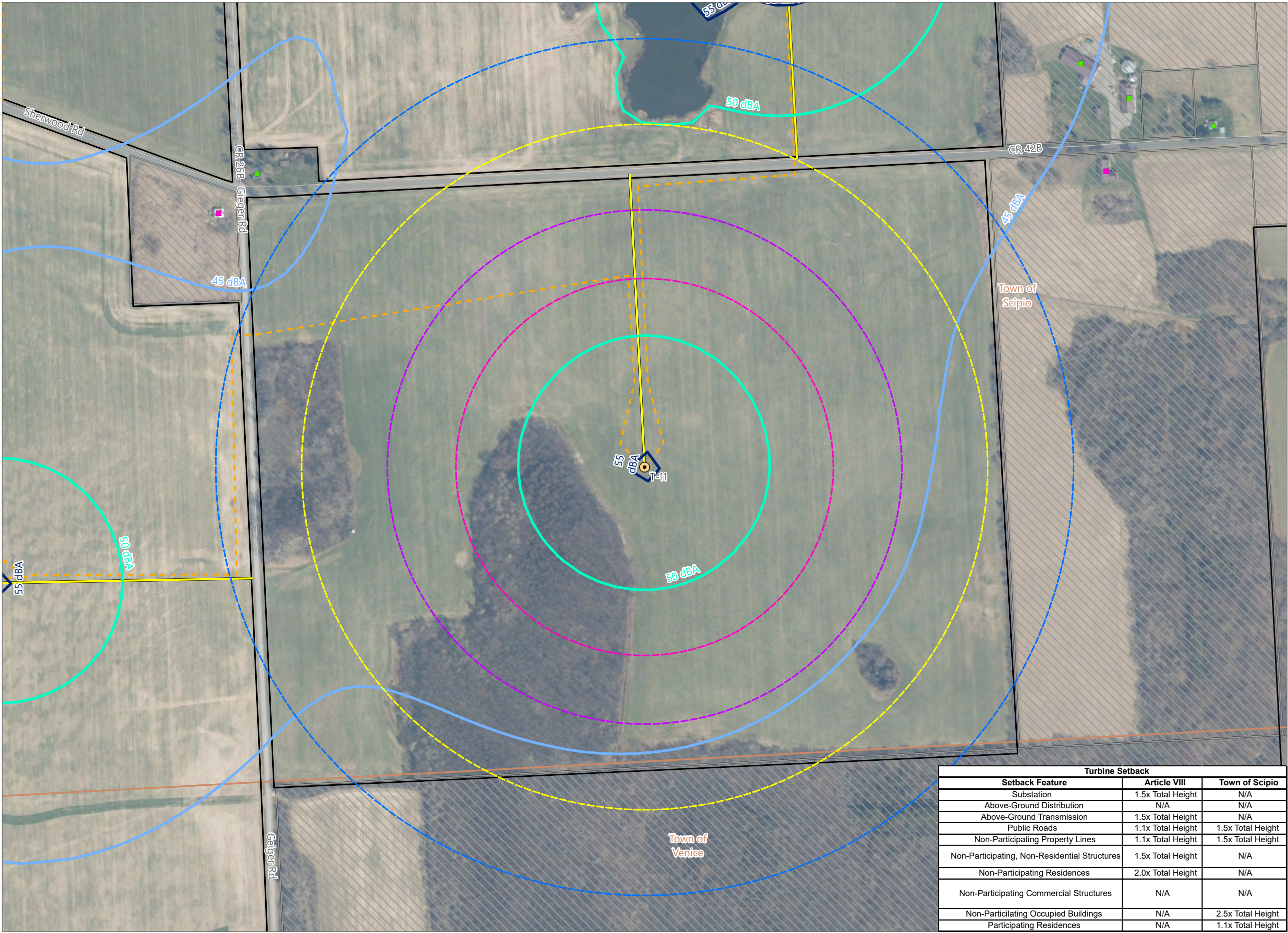
Figure 24-1. Setbacks
