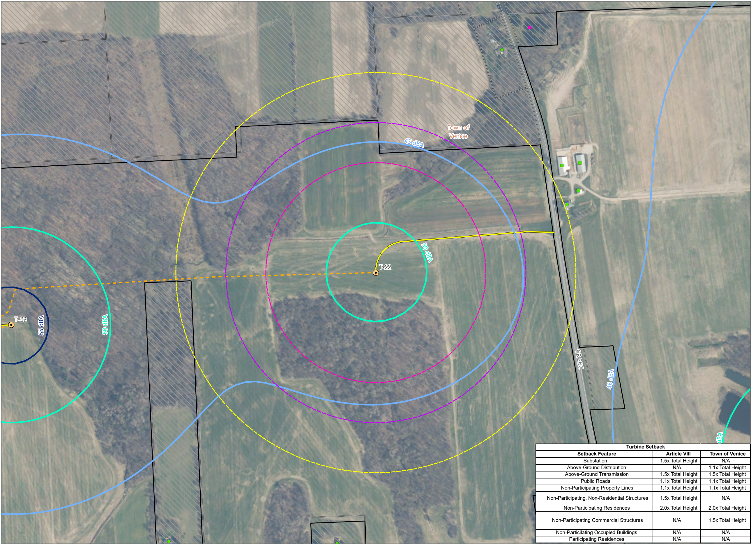
Figure 24-1. Setbacks
