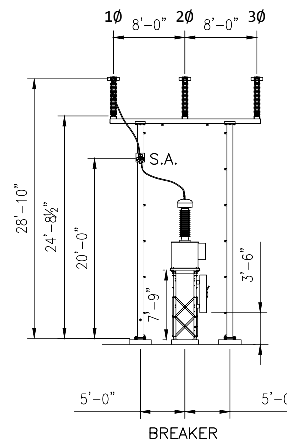
ELEVATION E-E
