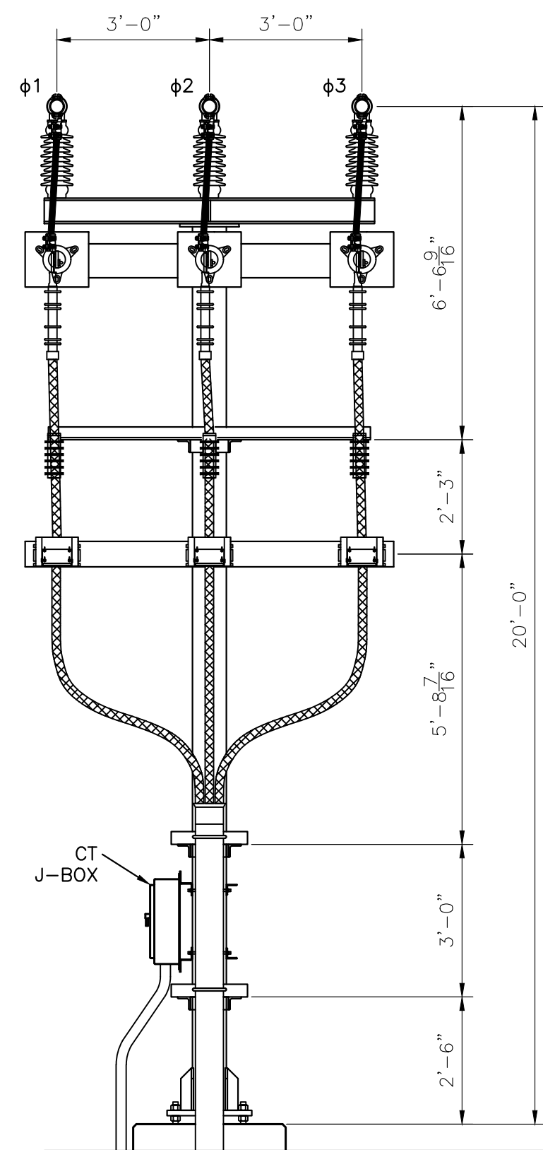
34.5kV CAP BANK 2 RISER, CT's AND SURGE ARRESTERS
