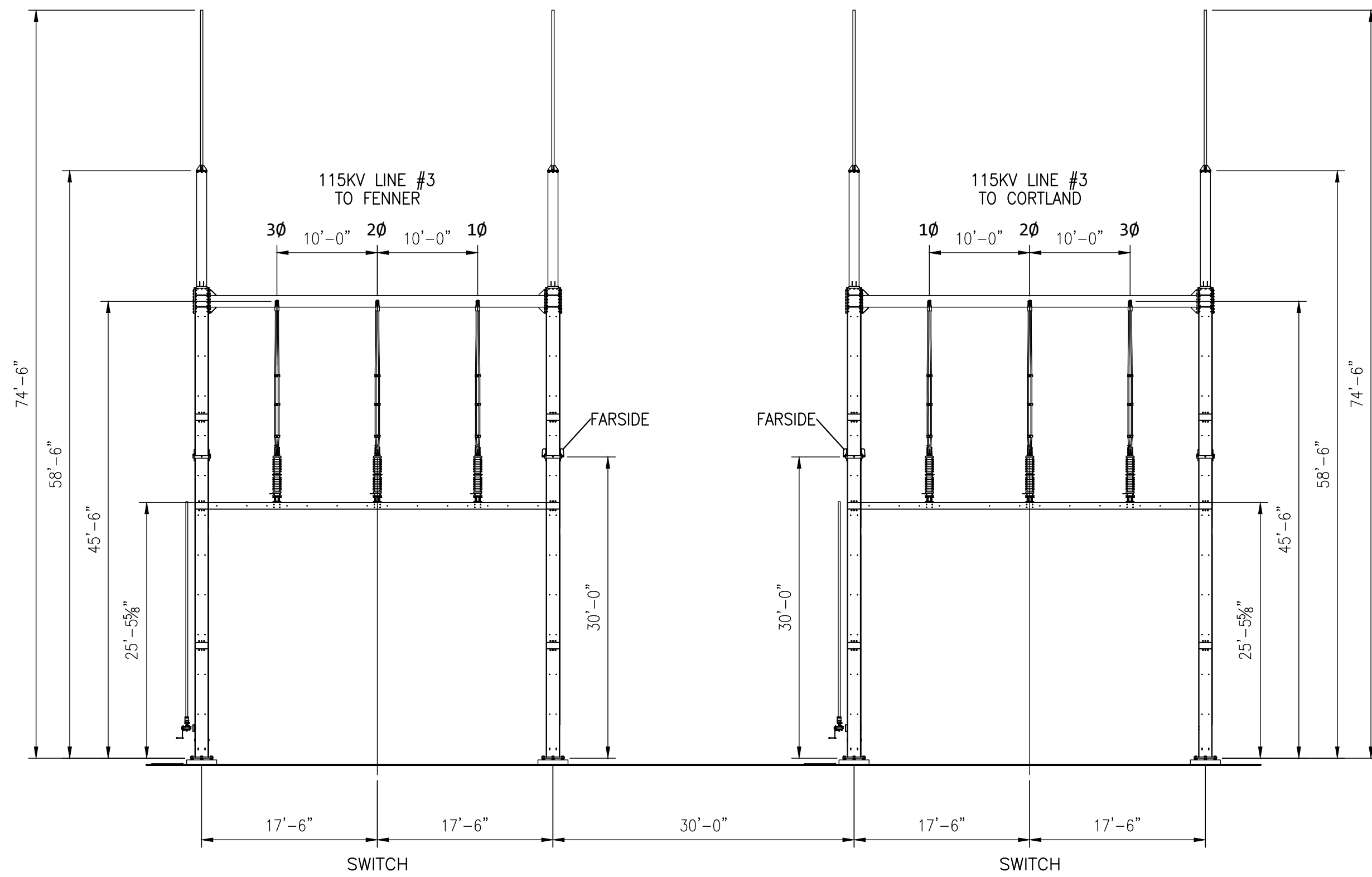
ELEVATION F-F
