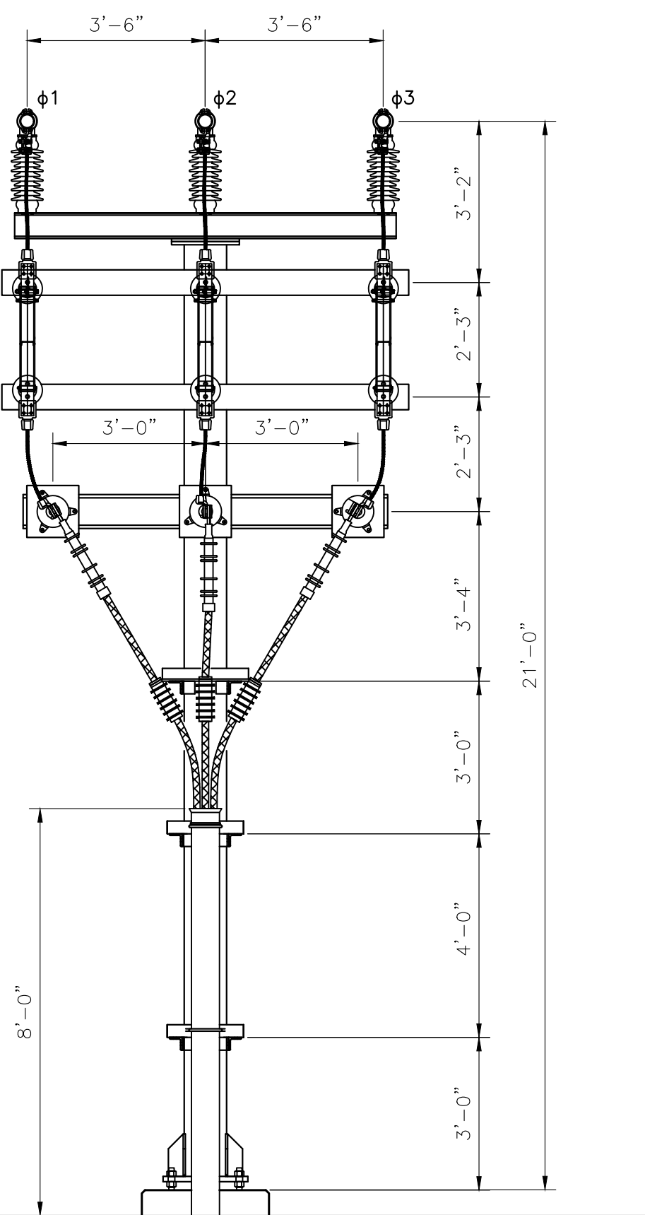
34.5kV FEEDER 12, SURGE ARRESTERS & HOOKSTICK SW. 89-122A
