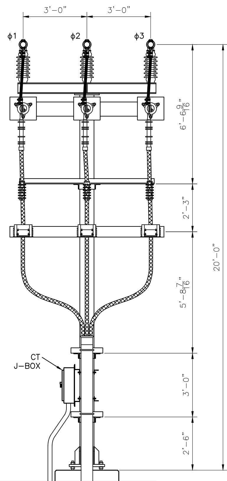
34.5kV CAP BANK 1 RISER, CT's AND SURGE ARRESTERS
