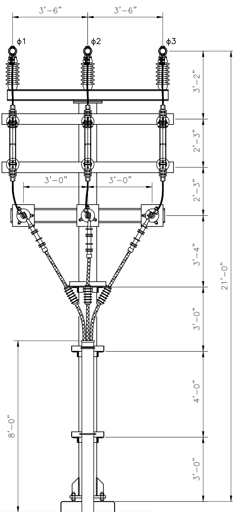
34.5kV FEEDER 11A, SURGE ARRESTERS & HOOKSTICK SW. 89-112A
