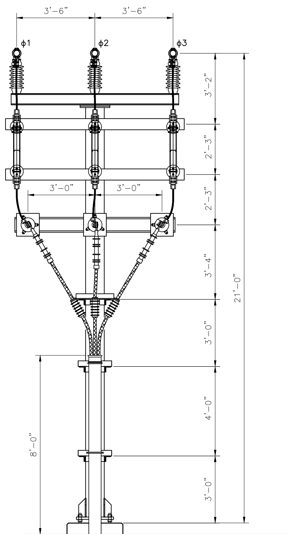
34.5kV CAP BANK 1 FEEDER, SURGE ARRESTERS & HOOKSTICK SW. 89-C1
