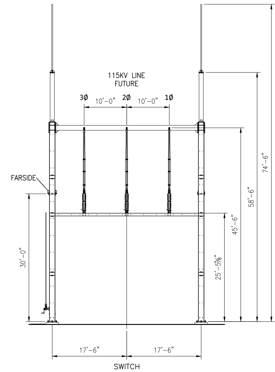
ELEVATION H-H
