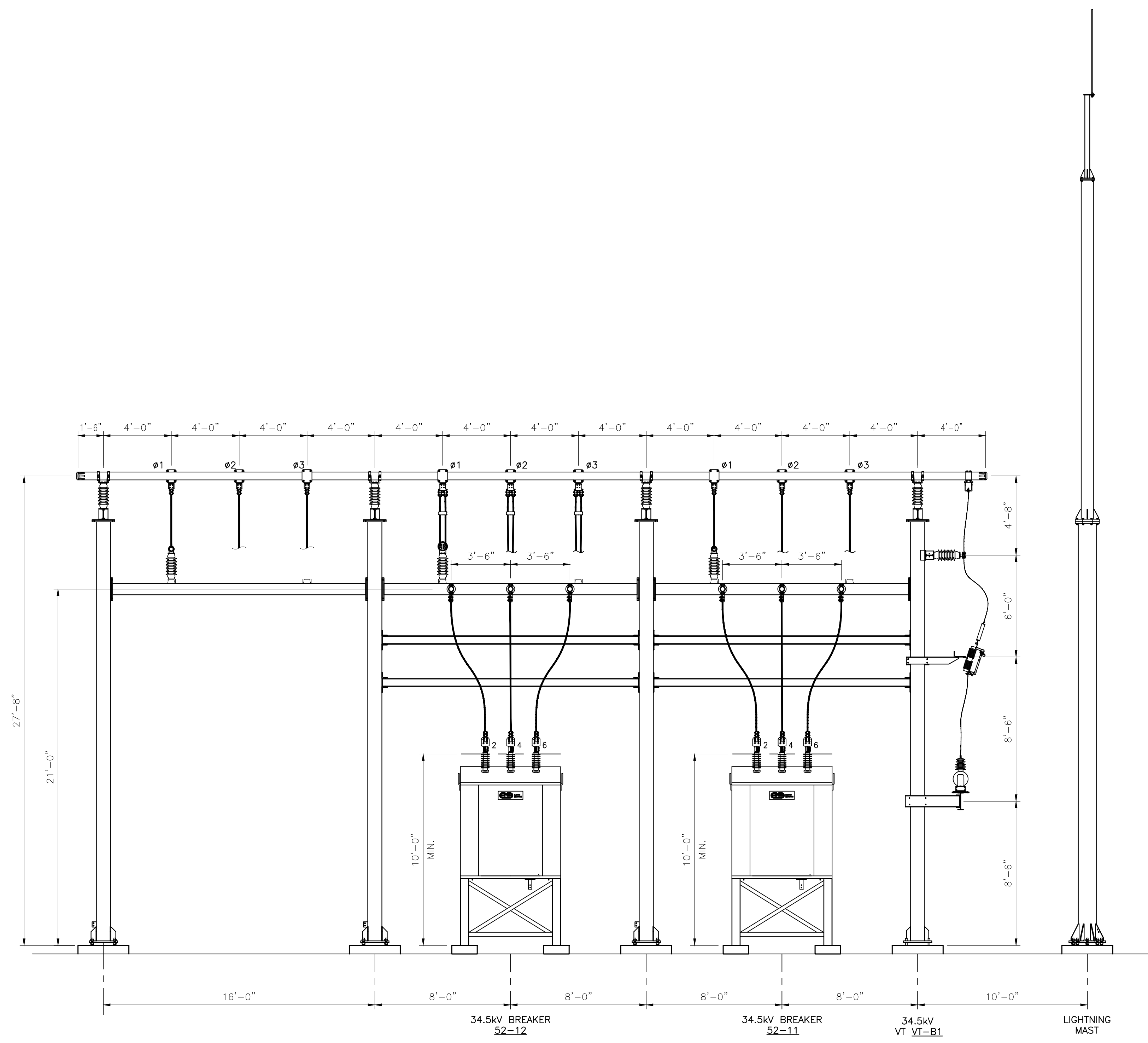
ELEVATION E-E
