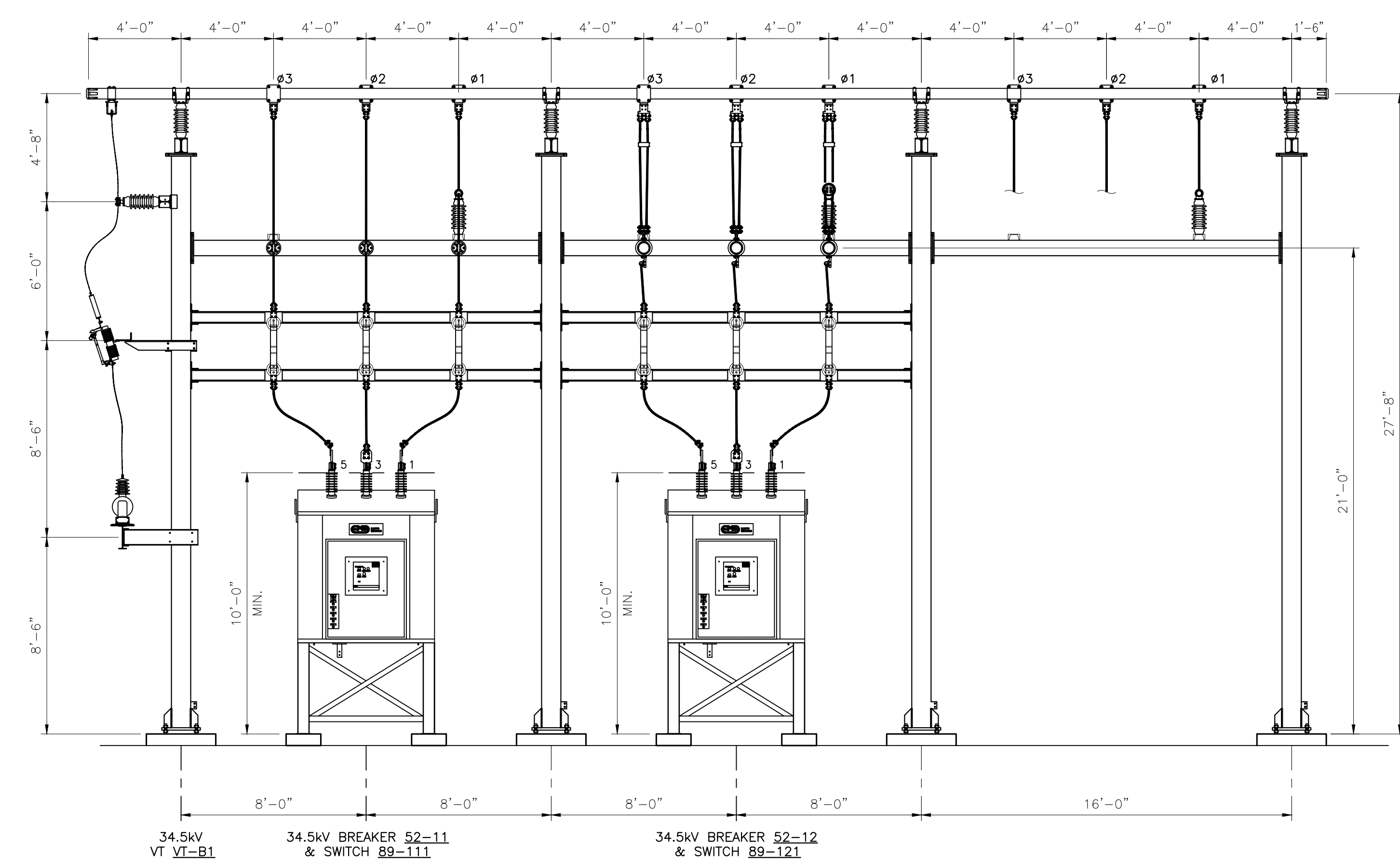
ELEVATION F-F (LIGHTNING MAST NOT SHOWN)
