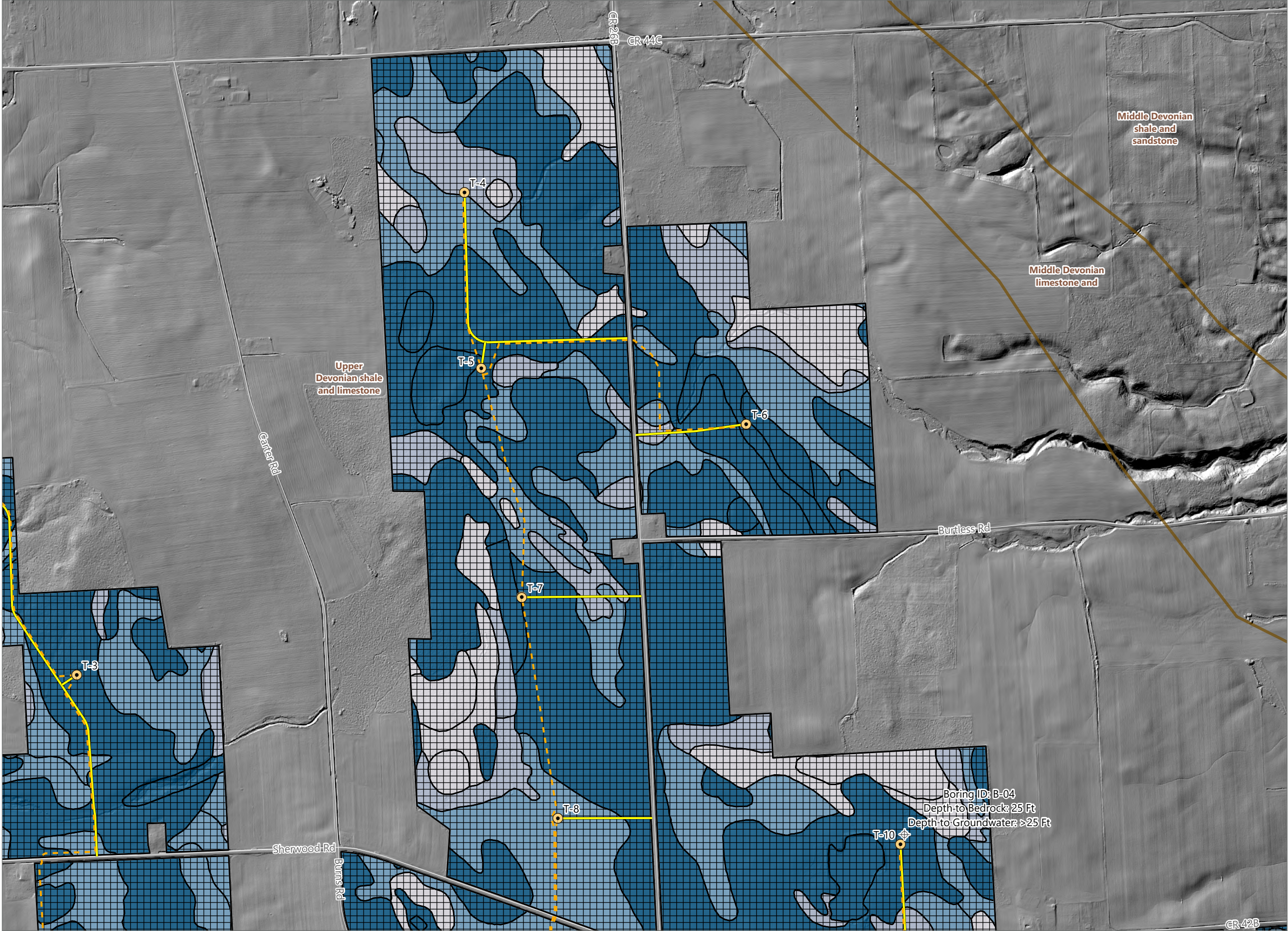
Figure 10-4. Bedrock
