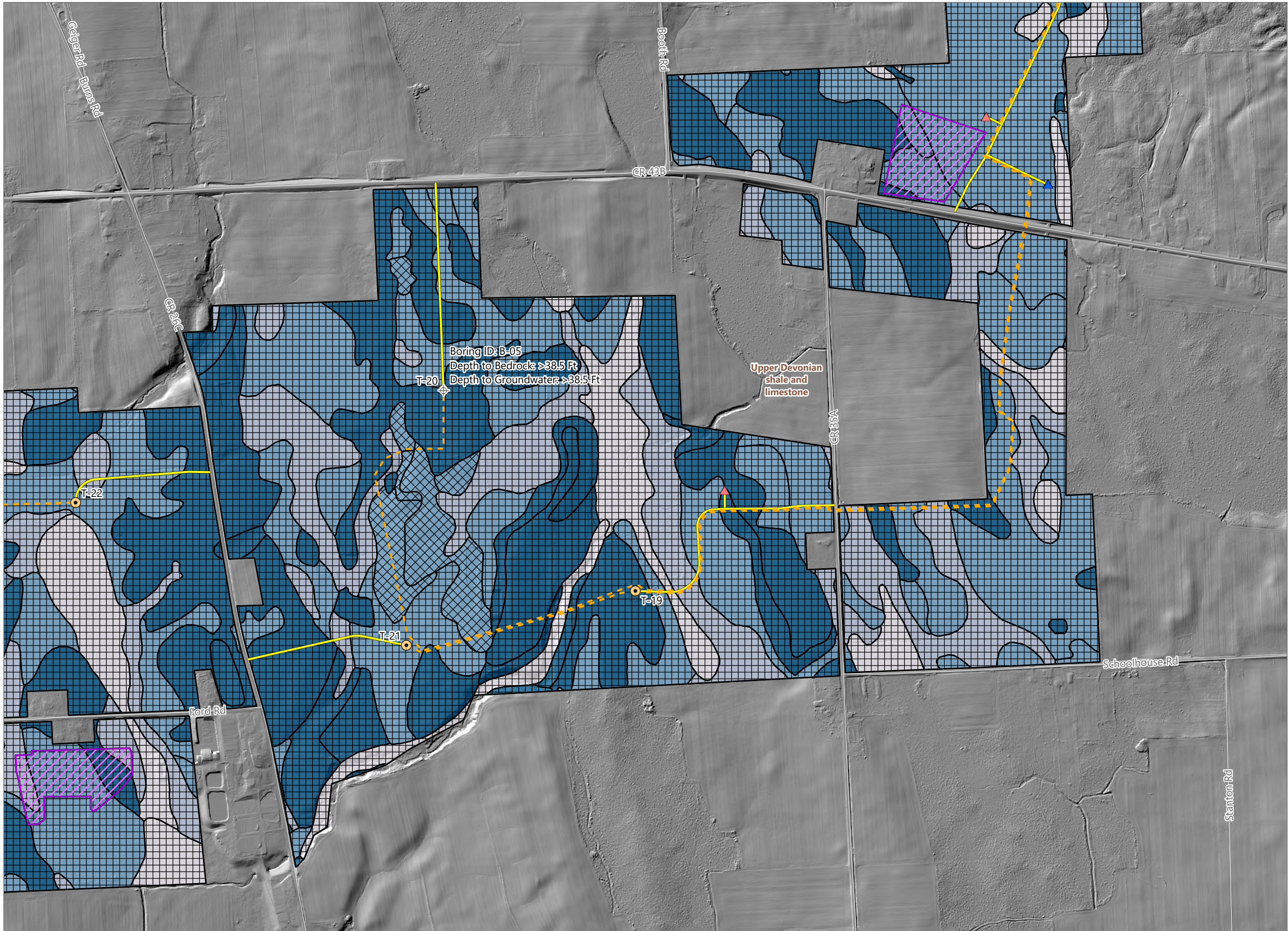
Figure 10-4. Bedrock
