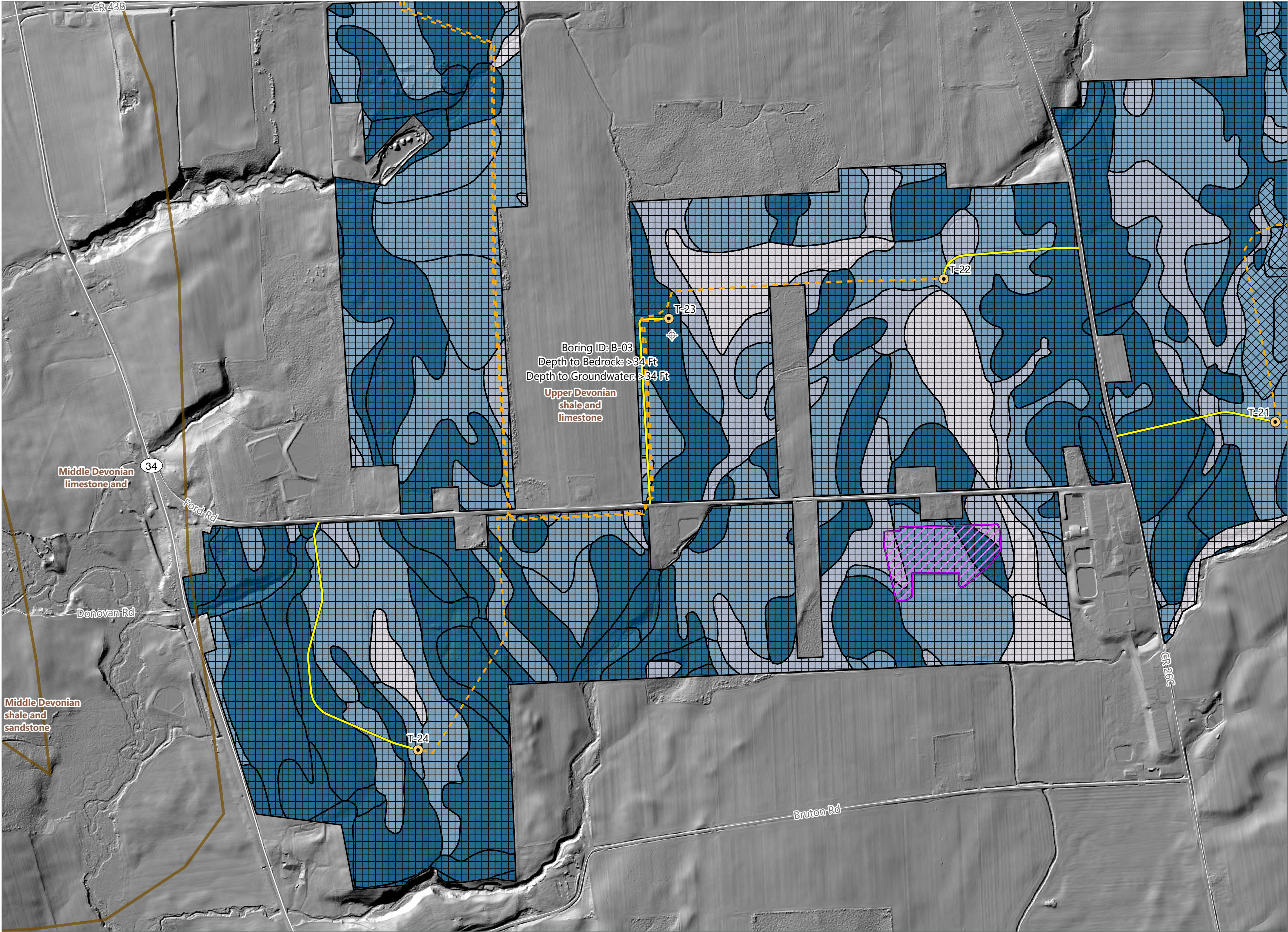
Figure 10-4. Bedrock
