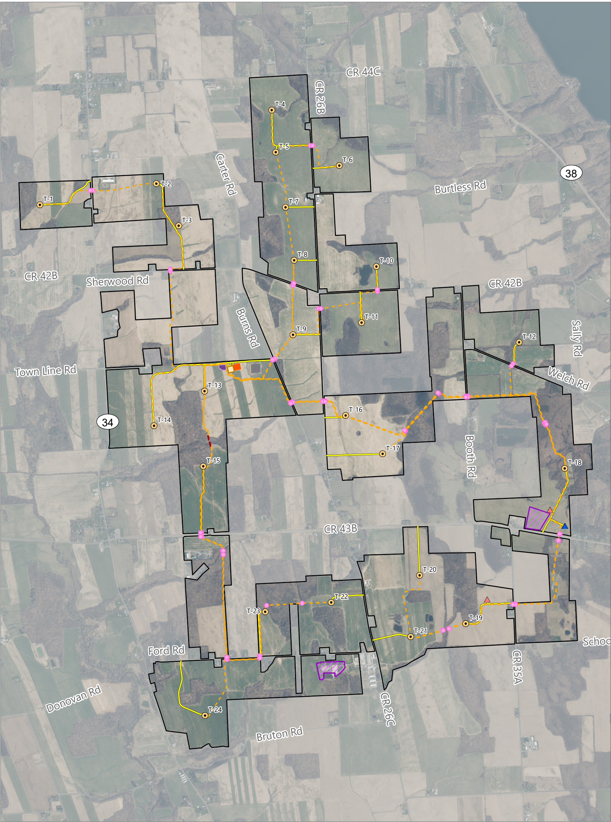
Figure 10-2. Trenchless Installation Locations
