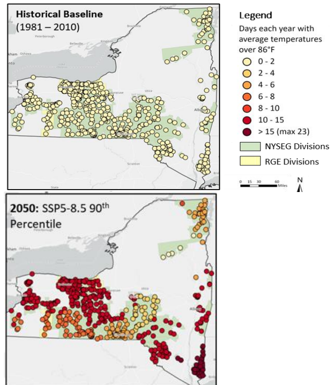
Figure 1. Historical and projected number of days with temperatures over 86°F in the service area
