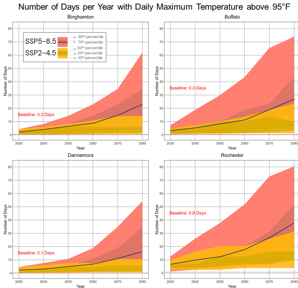
Figure 9. Average annual number of days that maximum temperature exceeds 95°F (35°C) for four representative weather stations for the 2030 to 2080 period.
