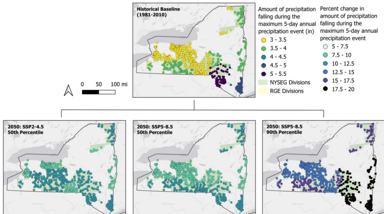
Figure 14. Average amount of precipitation at substations during the maximum 5-day precipitation event during a baseline period from 1981 to 2010 (top).
