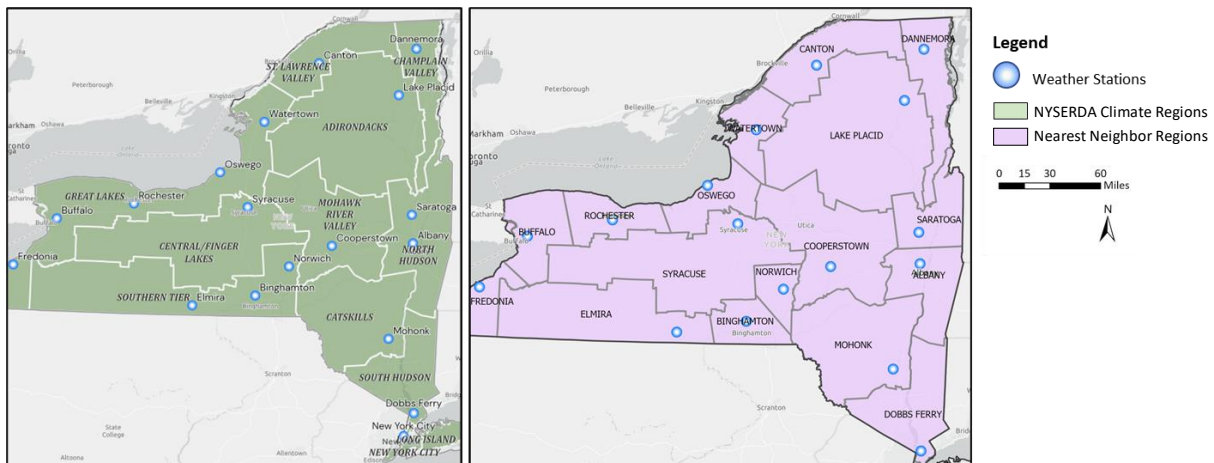
Figure 12. Weather stations and NYSEDA climate regions (left) and weather stations and polygons representing the area closest to each weather station within each NYSEDA climate region (right).
