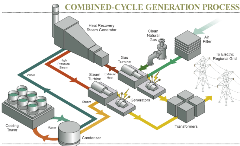
Figure 12: Combined Cycle Process Flow
