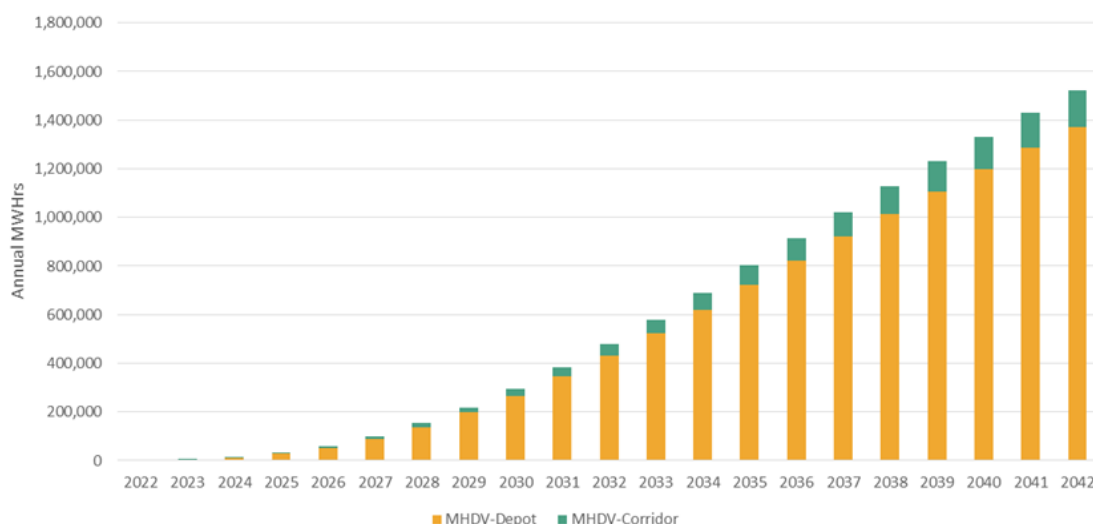
Figure C-11. Projected Load for MHDV Charging Energy– Most Likely Case
