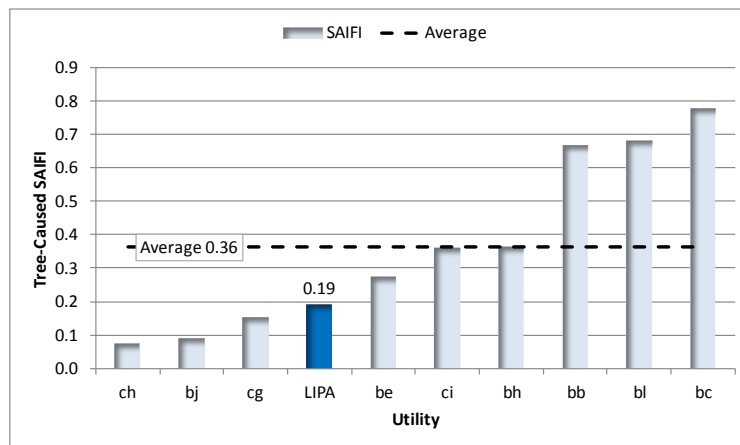
Figure 8. Tree-Caused System Average Interruption Frequency Index (SAIFI).
