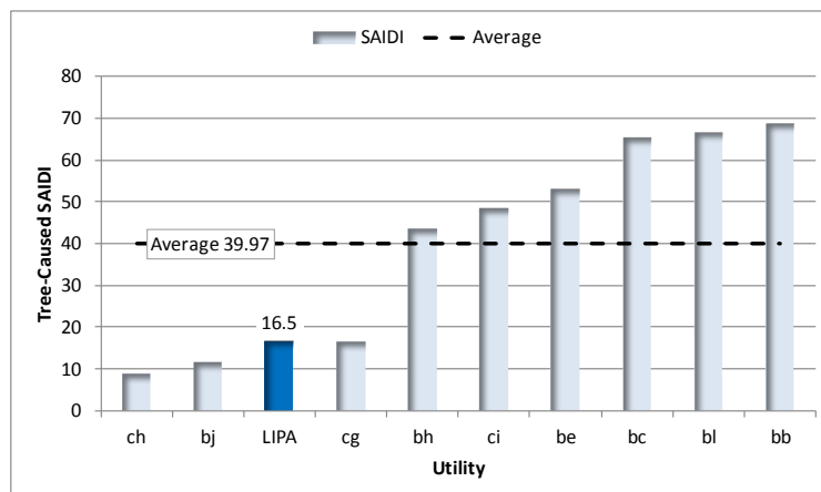
Figure 9. Tree-Caused System Average Interruption Duration Index (SAIDI).
