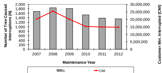
Figure 3d. Five year Trend in Number (N) of Tree-Caused Interrupted and Customers Min. Interrupted (CMI) on All Overhead Lines 4 .
