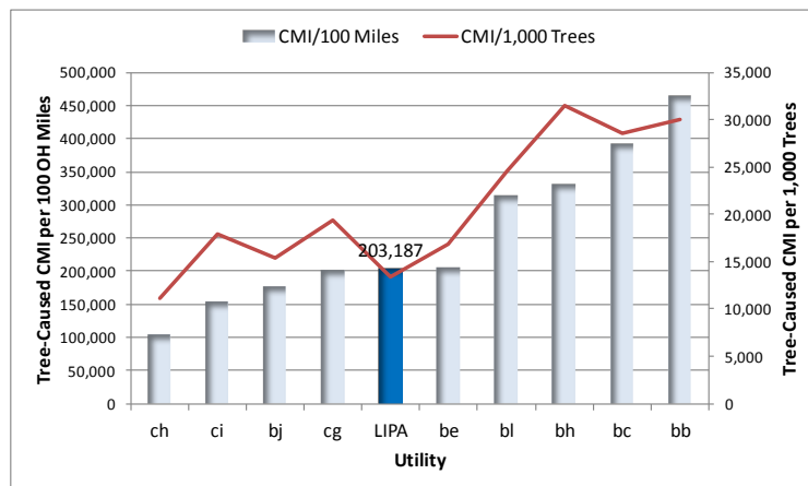
Figure 8. Customer Minutes Interrupted (CMI) per 100 Overhead Miles.
