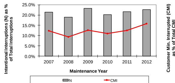
Figure 3e. Five-year Trend in Number (N) and Customers Minutes Interrupted (CMI) on All Overhead Lines due to Intentional Interruptions Expressed as Percentage of All Tree-caused Interruptions (Excluding Storms).
