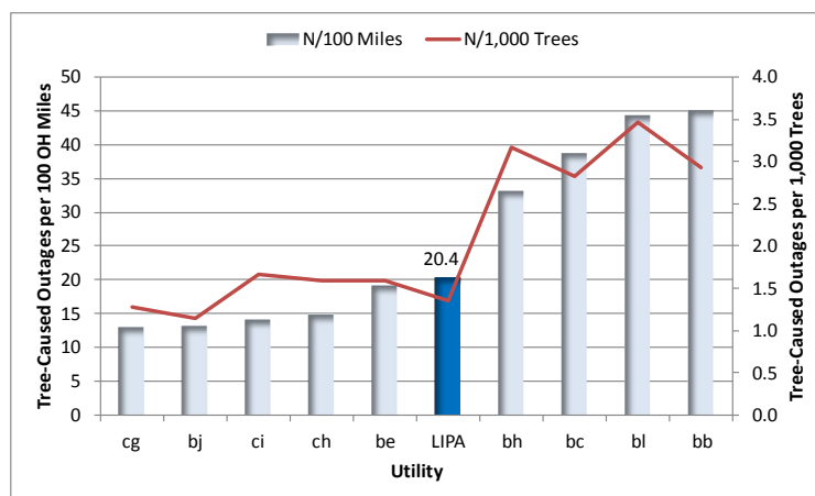
Figure 6. Number (N) of Tree Caused events per 100 Overhead Miles.
