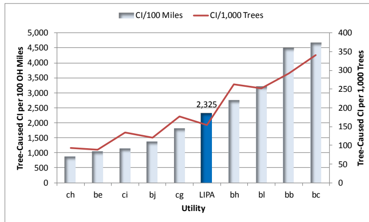
Figure 7. Customers Interrupted (CI) per 100 Overhead Miles.
