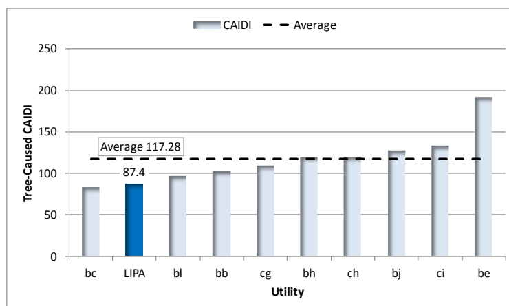
Figure 10. Tree-Caused Customer Average Interruption Duration Index (CAIDI).
