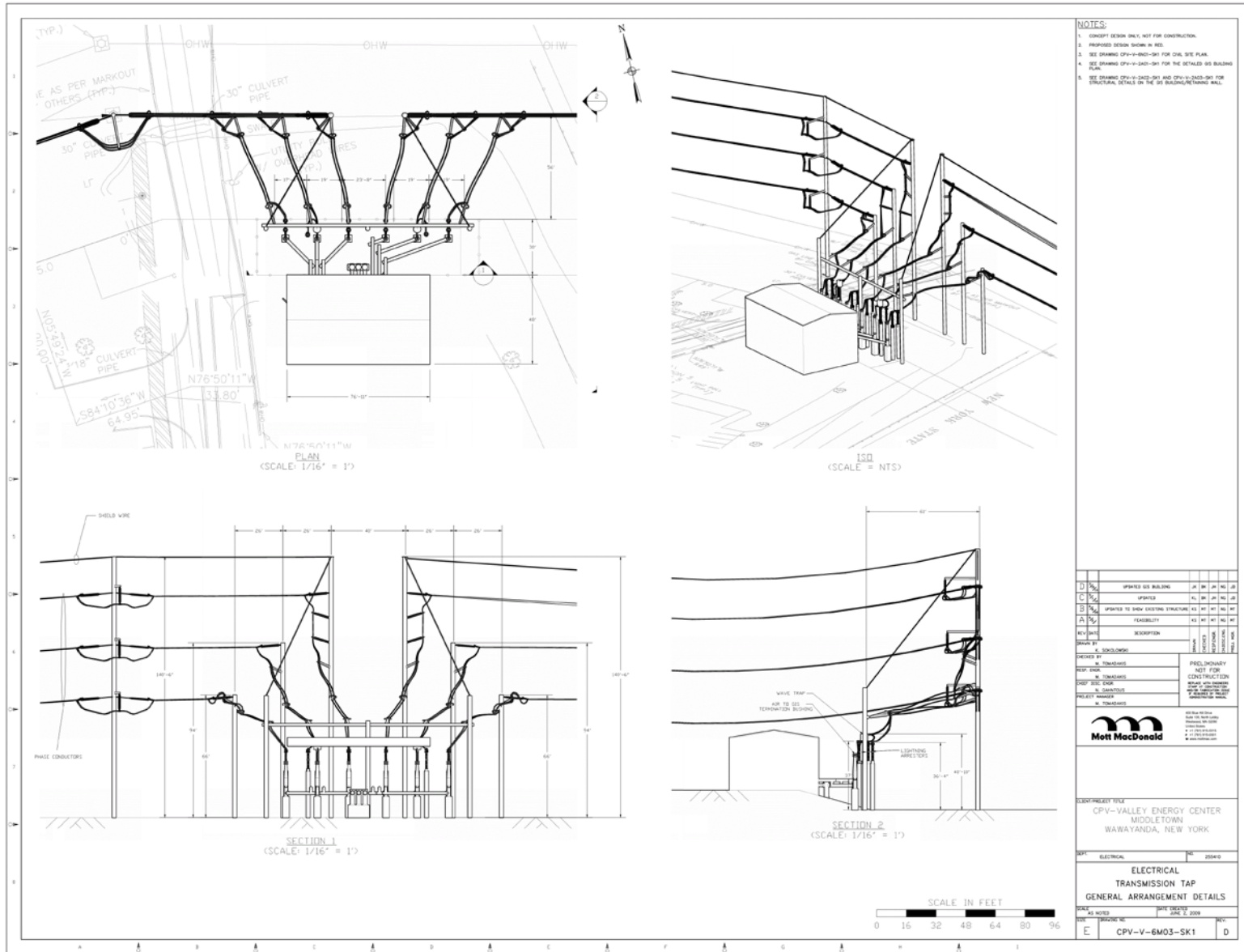
Figure C-2 (GIS Building Plan and Elevation)
