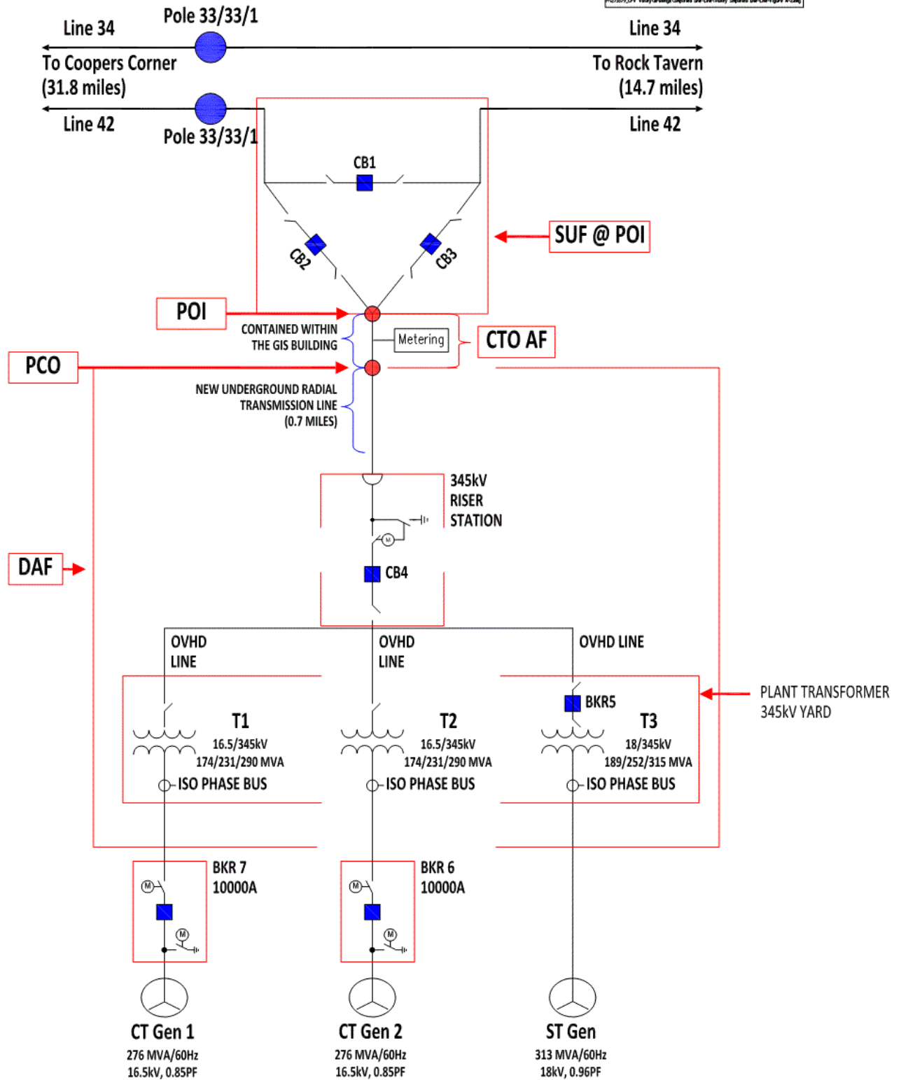
Figure A-2 CPV Valley Energy Center One-Line
