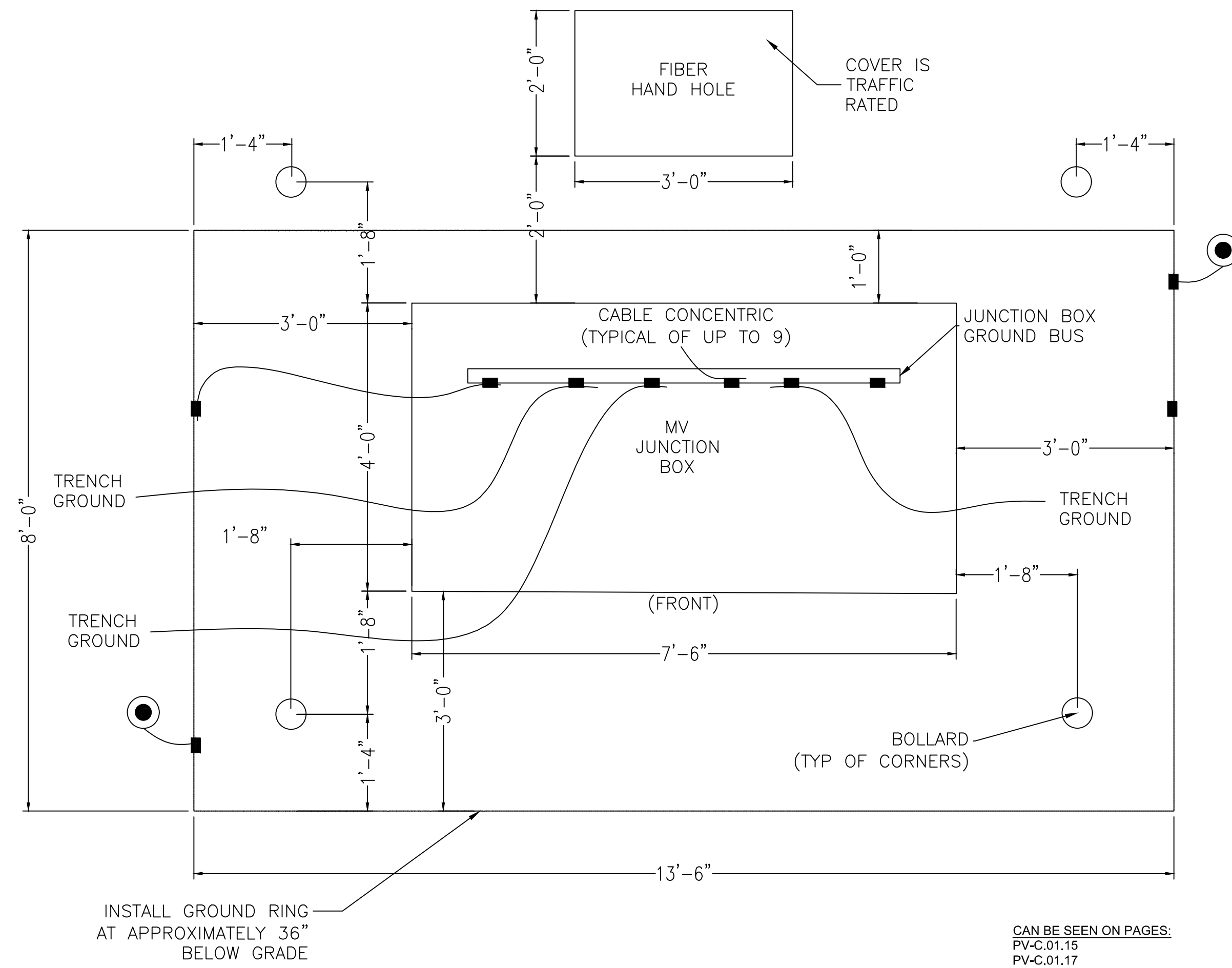
1 TYPICAL JUNCTION BOX PLAN VIEW SCALE: N.T.S.
