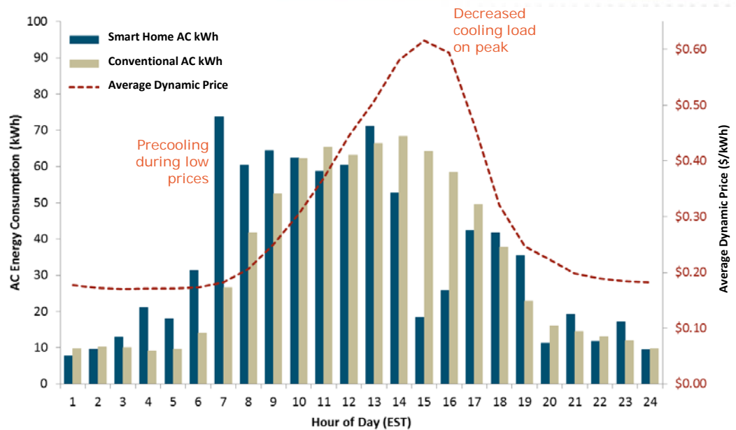
Figure 53: Smart vs. conventional air conditioner energy usage in response to an hourly dynamic price.
