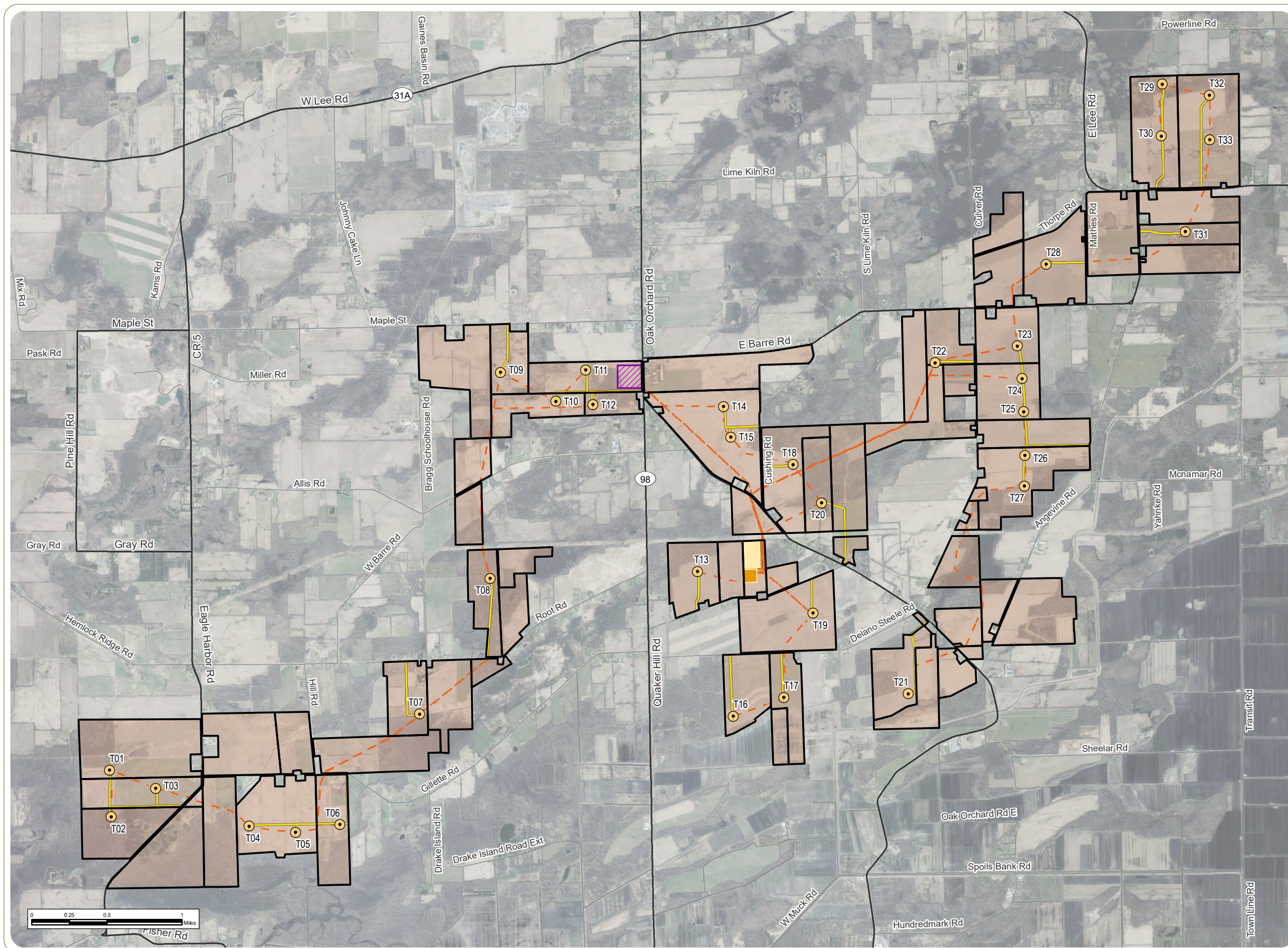
Figure 3: Preliminary Facility Layout
