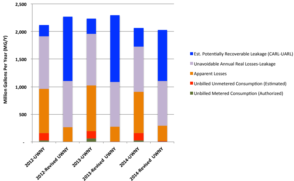
Figure 2-4. Comparison of Estimated Potentially Recoverable Leakage and NRW Components Based on Calculations Using Data in UWNY and Revised UWNY AWWA Water Audits, 2012-2014
