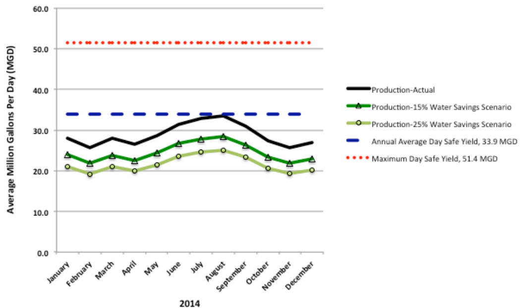
Figure ES-1. UWNY Water Production Scenarios With 15% and 25% Savings From System Leakage & Customer Conservation in 2014
