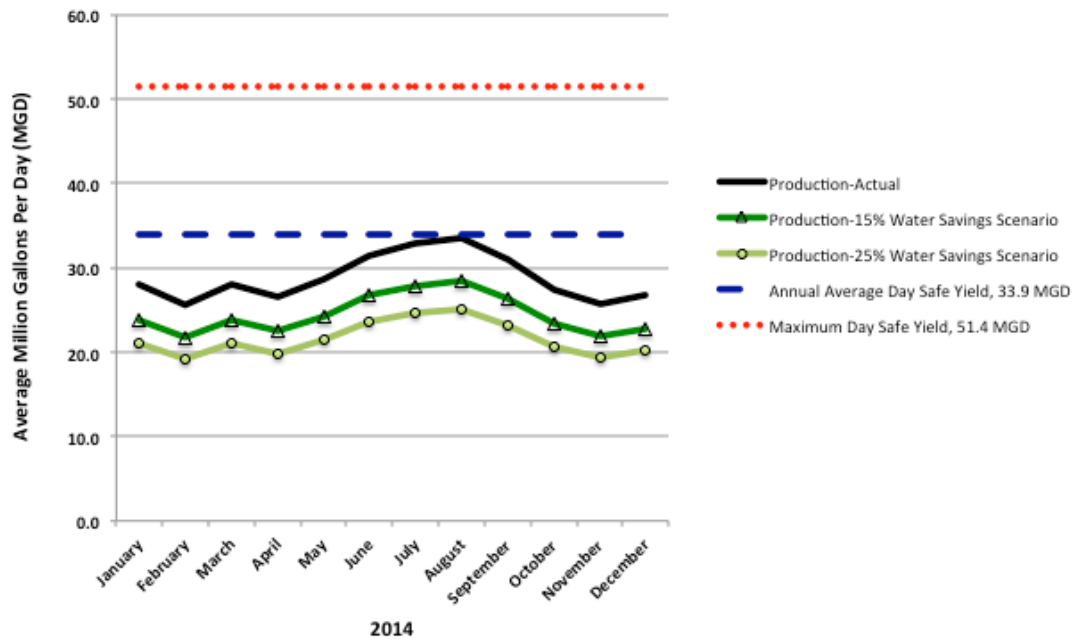
Figure 4-1. UWNY Water Production Scenarios With 15% and 25% Savings From System Leakage & Customer Conservation in 2014
