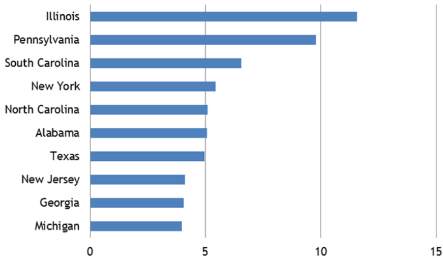
EXHIBIT 5-2. NUCLEAR CAPACITY FOR TOP TEN U.S. STATES, 2015, GIGAWATTS 75
