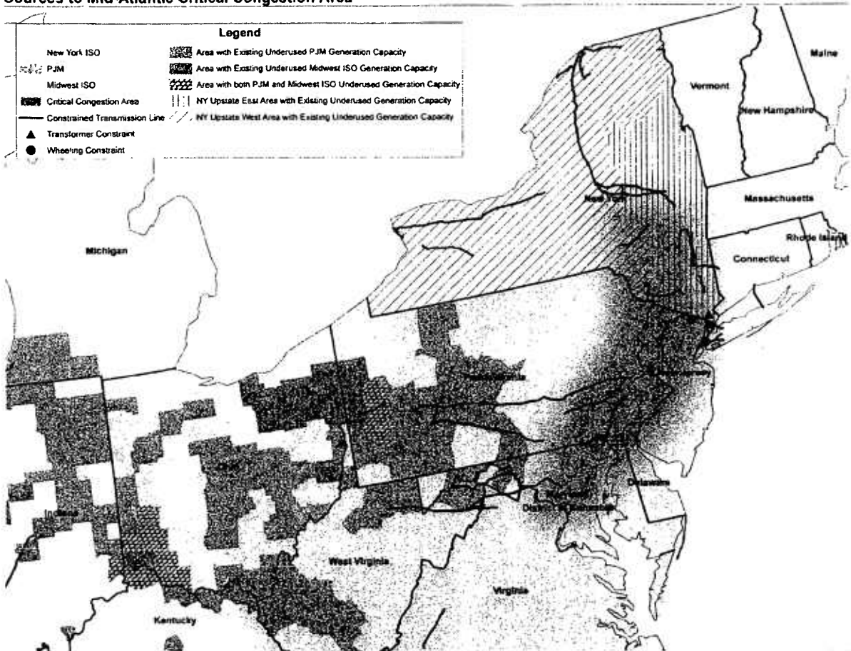
Figure VIII-16. Key Transmission Constraints Preventing Electricity Transfers from Available Lower-Cost Generation Sources to Mid-Atlantic Critical Congestion Area
