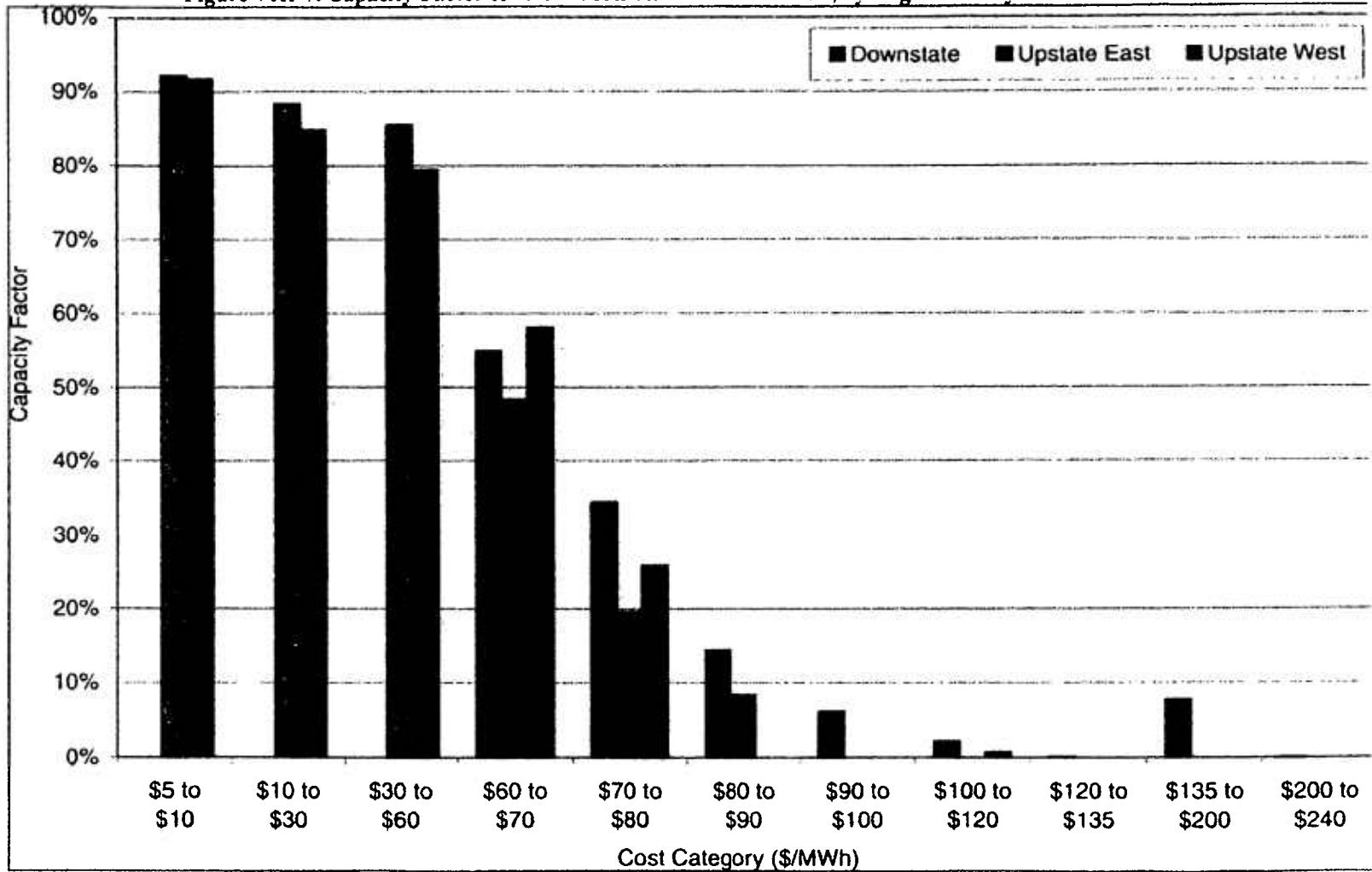
Figure VIII-7. Capacity Factor for New York State Thermal Units, by Region and by Production Cost Class
