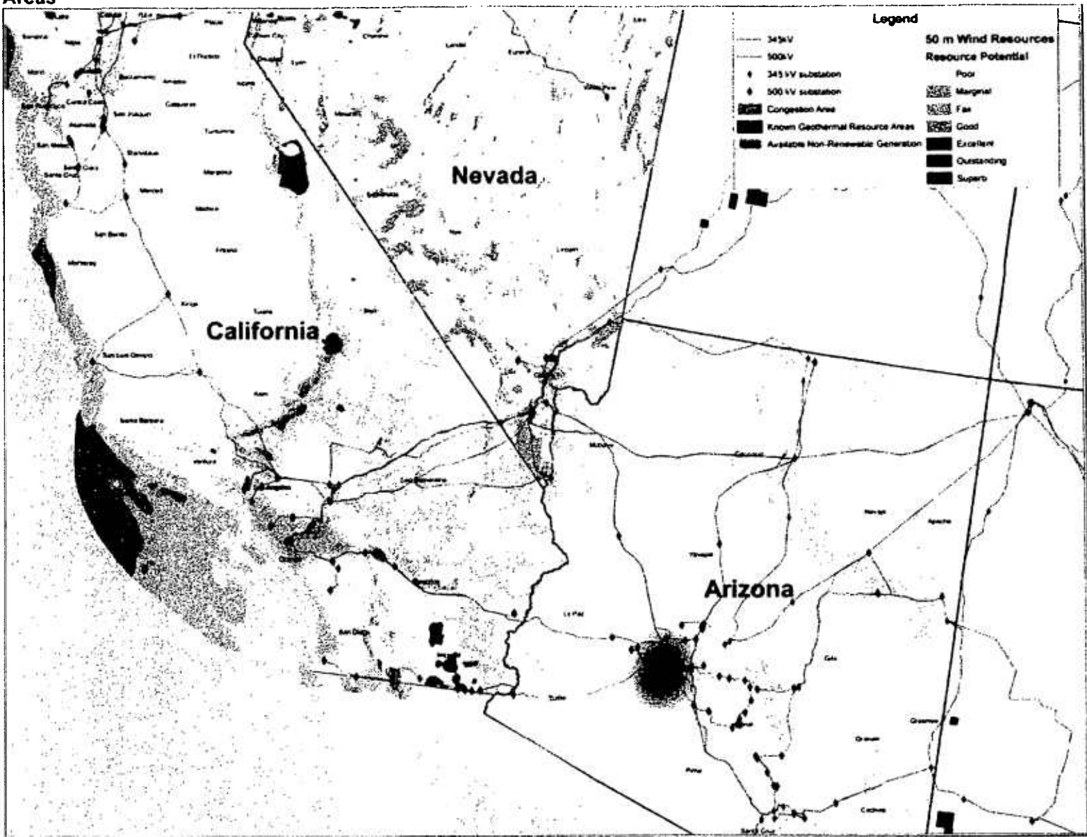
Figure IX-5. Southern California Critical Congestion Area and Potential Gas-fired, Wind and Geothermal Generation Source Areas
