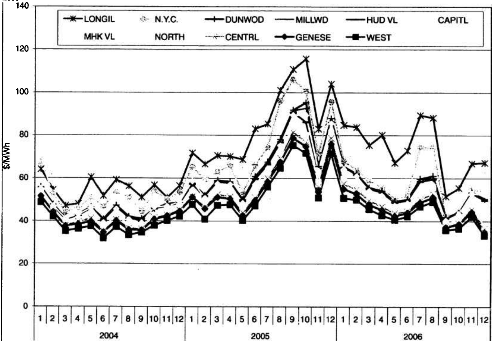
Figure VIII-12. Historical Round-the-Clock Monthly Day-Ahead LBMPs in New York ISO, by Zone, January 2004-December 2006
