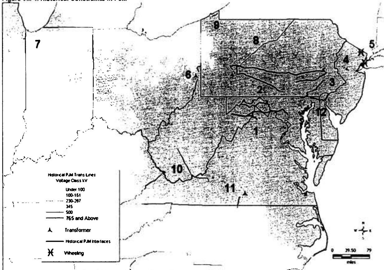
Figure VIII-1. Historical Constraints in PJM
