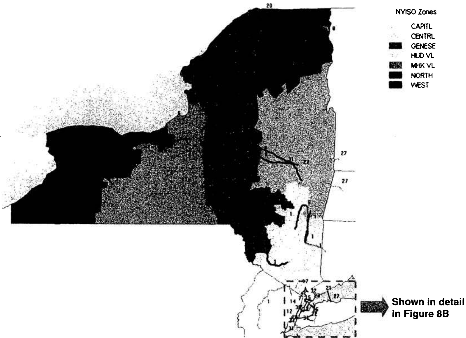
Figure VIII-8A. Transmission Constraints Limiting the Ability to Use Generation in Upstate New York and Ontario to Serve Downstate New York Loads
