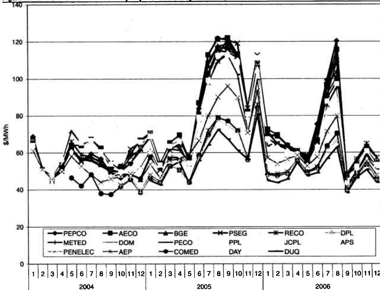
Figure VIII-10. Historical On-Peak Monthly Day-Ahead LMPs by PJM Zone, 2004-2006
