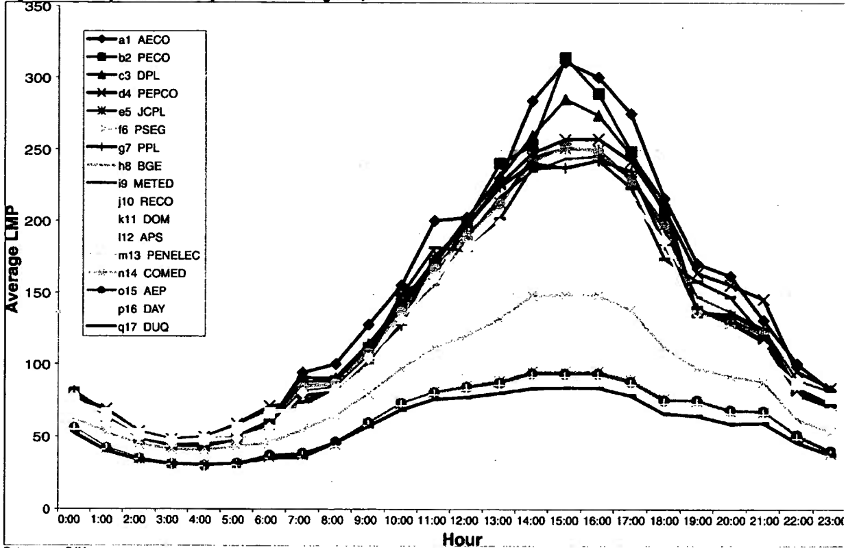
Figure VIII-11. Day-Ahead LMPs by PJM Zone on August 8, 2005
