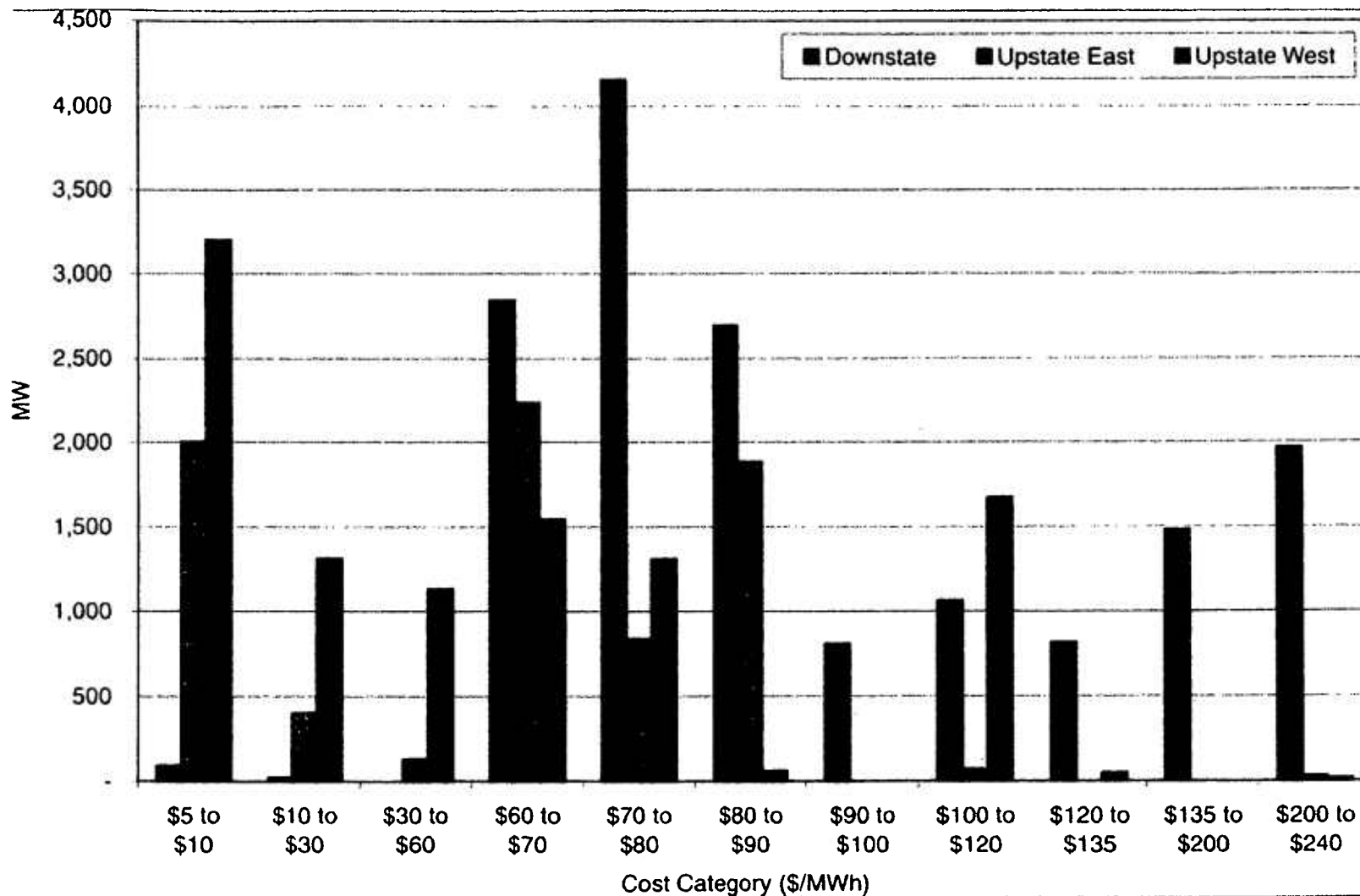
Figure VIII-6. New York State Installed Thermal Capacity by Region and by Production Cost Class
