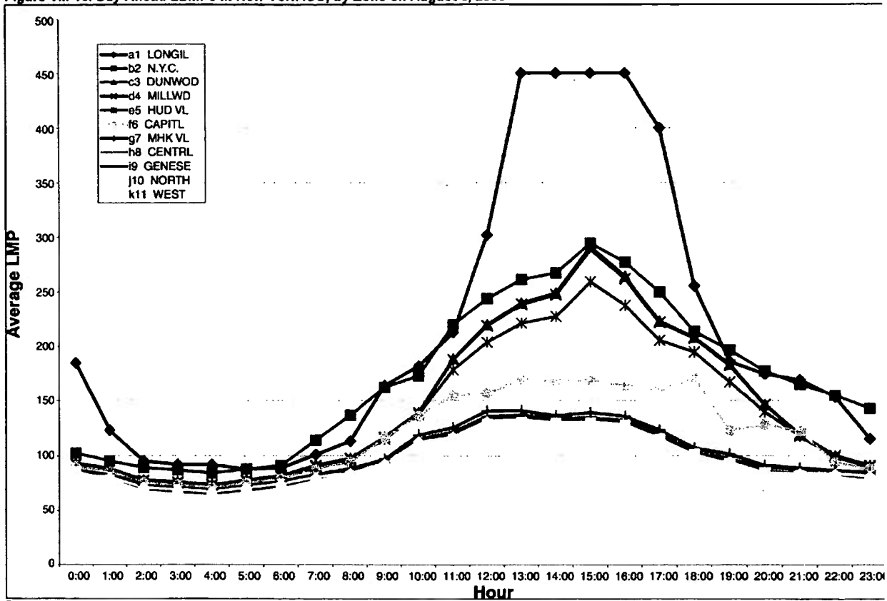
Figure VIII-13. Day-Ahead LBMPs in New York ISO, by Zone on August 5, 2005
