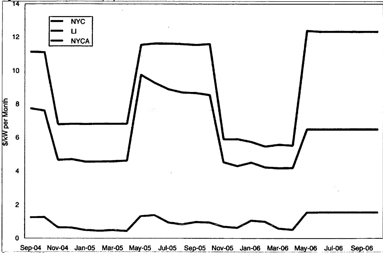
Figure VIII-14. UCAP Auction Prices, September 2004-October 2006
