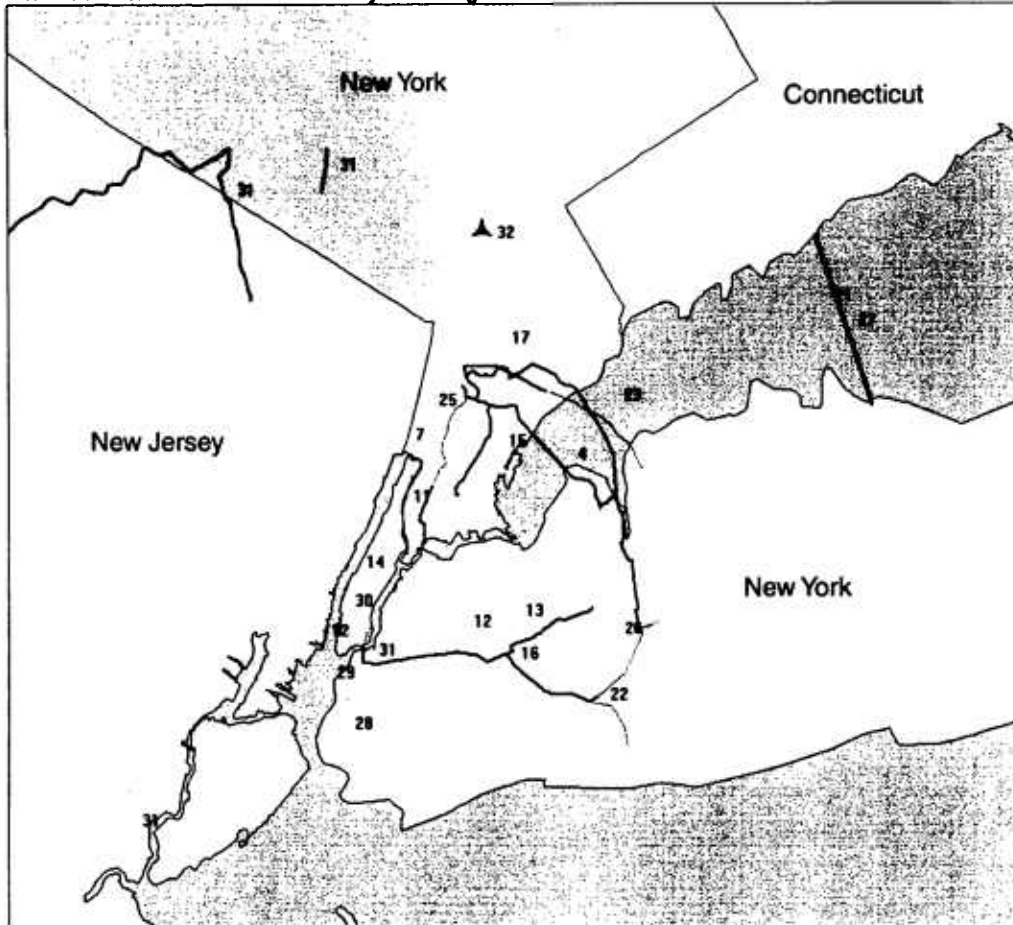
Figure VIII-8B. Transmission Constraints in New York City Area Limiting the Ability to Use Generation in Upstate New York and Ontario to Serve Loads in the City and Long Island
