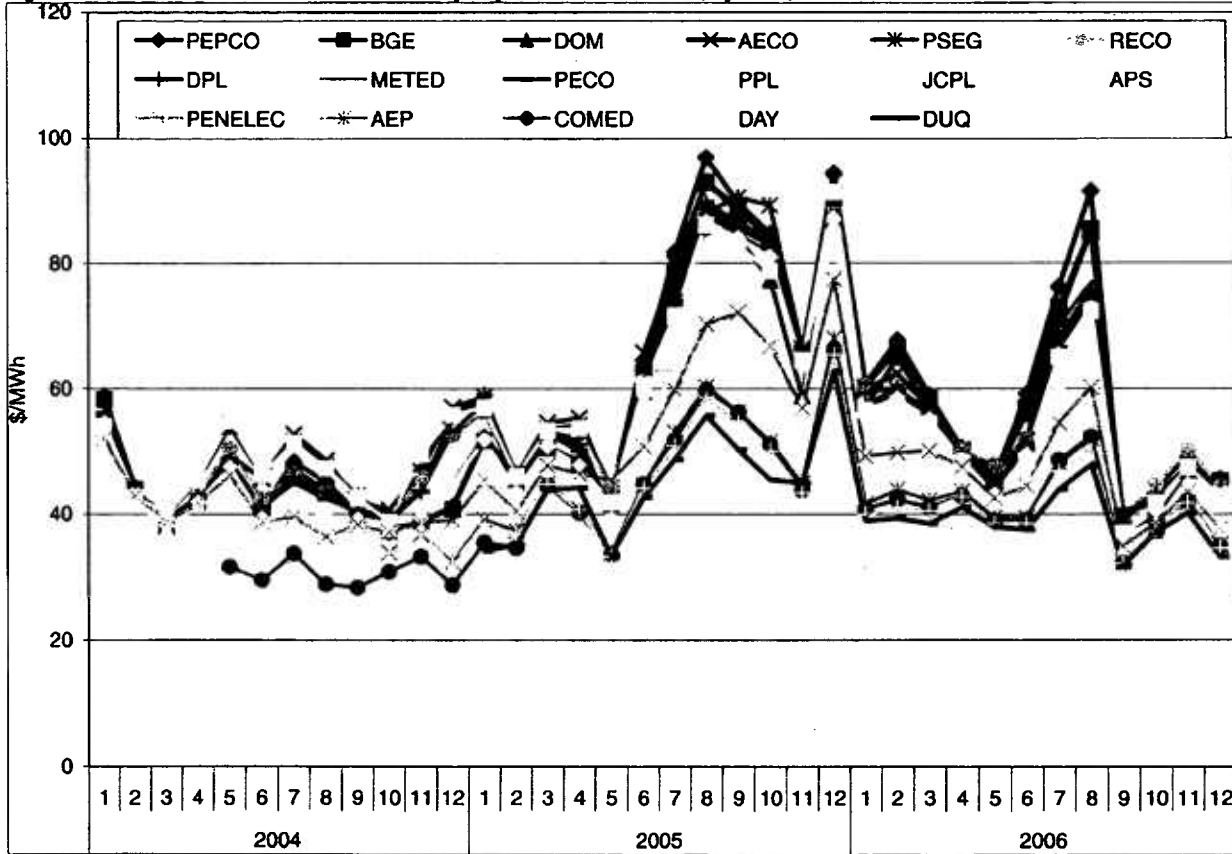
Figure VIII-9. Historical Round-the-Clock Monthly Day-Ahead LMPs in PJM, by Zone, 2004-2006
